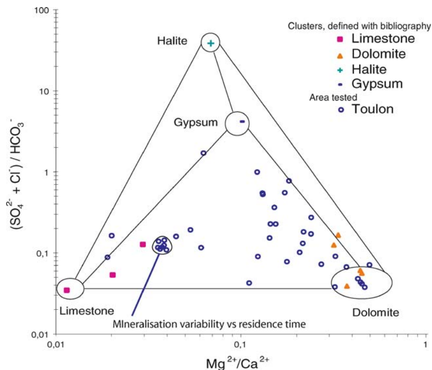
Fig. 7 Component mixture of karst water chemistry. Evolution of the ratio Mg^{2+}/Ca^{2+} and (SO_4^{2-}+Cl^-)/HCO_3^- . The clusters were built with data from Cova and Durozoy (1980), Laly (1981), Vernet and Vernet (1981), Puig (1987), Petelet et al. (1998), Emily (2000), Fairchild et al. (2000) and Reynaud (2000). The plotted data correspond to the Siou-Blanc spring measurements
