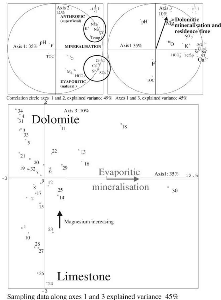
Fig. 8 Principal component analysis of water chemistry measurements at the Siou-Blanc springs
