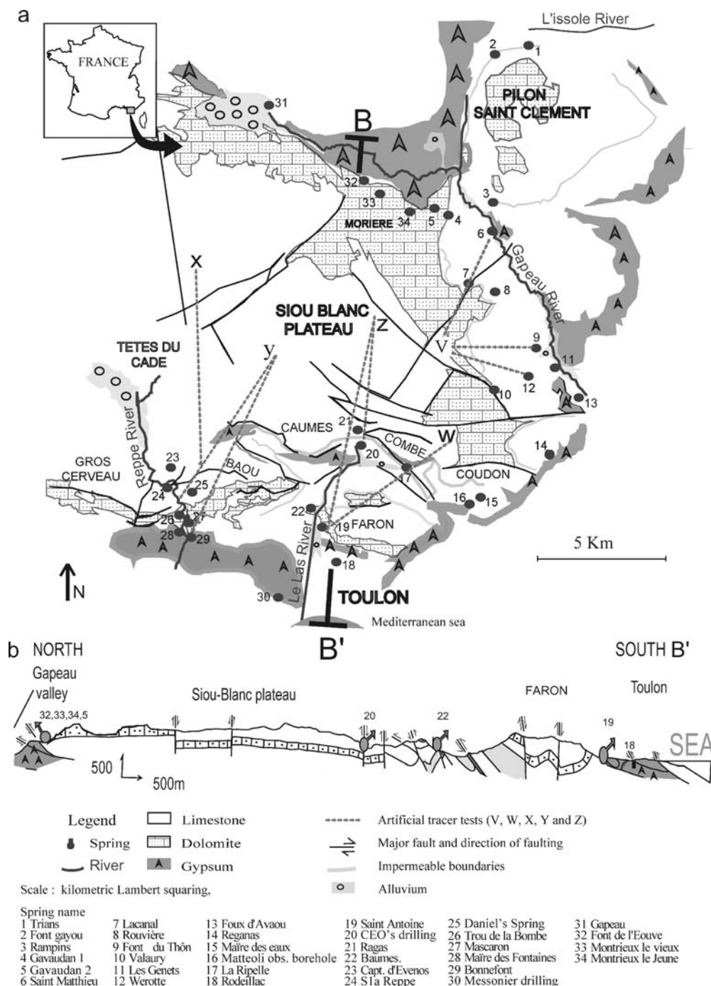
Fig. 3 a Hydrogeological map and b cross section of the Siou-Blanc Plateau
