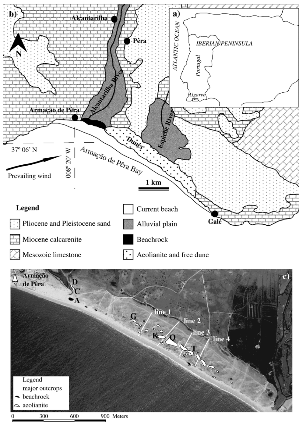
Fig. 1. (a) Location of the study area in the Algarve, southern Portugal; (b) Armção de Pêra Bay and dune field; (c) Georeferenced Ground Penetrating Radar (GPR) lines and aeolianite outcrops (see Fig. 4). Capital letters A, C, D, G, K, Q and T designate the outcrops from which samples were collected for textural analysis and radiocarbon dating.
