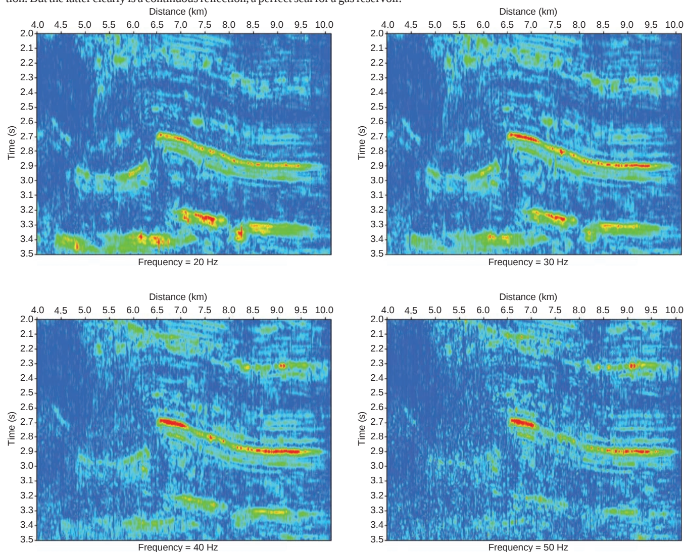
Figure 7. Constant-frequency profiles without inverse-Q filtering. The low-frequency shadow (at 3.0–3.4 s) underneath the carbonate gas reservoir appears in low frequency profiles (20 and 30 Hz) but gradually disappears from the high frequency profiles (40 and 50 Hz).
