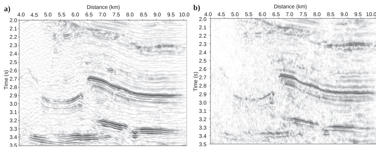
Figure 6. (a) The example seismic profile without inverse-Q filtering, and (b) the section after inverse-Q filtering. After inverse-Q filtering, the width of reflected wavelets becomes consistently narrow from shallow to deep. Many subtle faults appear above and beneath the target reflection. But the latter clearly is a continuous reflection, a perfect seal for a gas reservoir.
