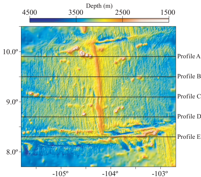
Figure 11. Location of the study area, where the profiles were taken from. Four of these profiles run across the mid-ocean ridge, and one is parallel to the transform fault. Location of the profiles is shown as thick black lines.
