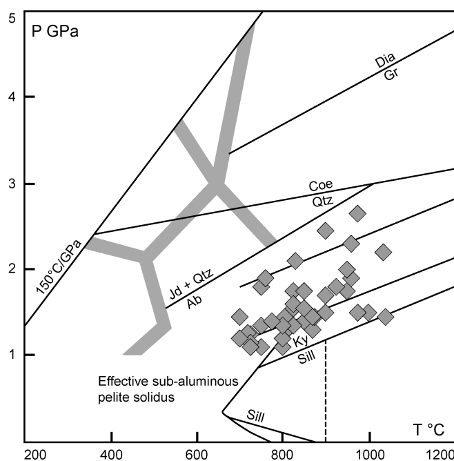
FIG. 5. Peak metamorphic P-T conditions of metamorphic belts: eclogite–high-pressure granulite (E-HPG) metamorphic belts (data from Table 3).
