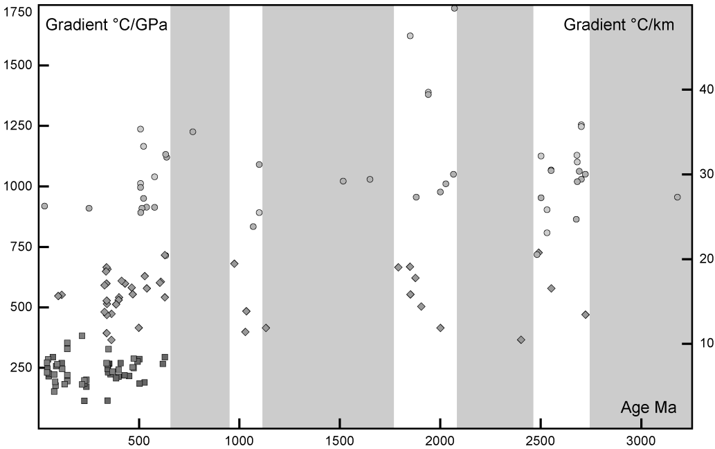
FIG. 8. Plot of thermal gradients versus age for the three main types of extreme metamorphic belt. Symbols: circles = G-UHT metamorphism; diamonds = E-HPG metamorphism; squares = HP-UHP metamorphism; data from Tables 1–5.
