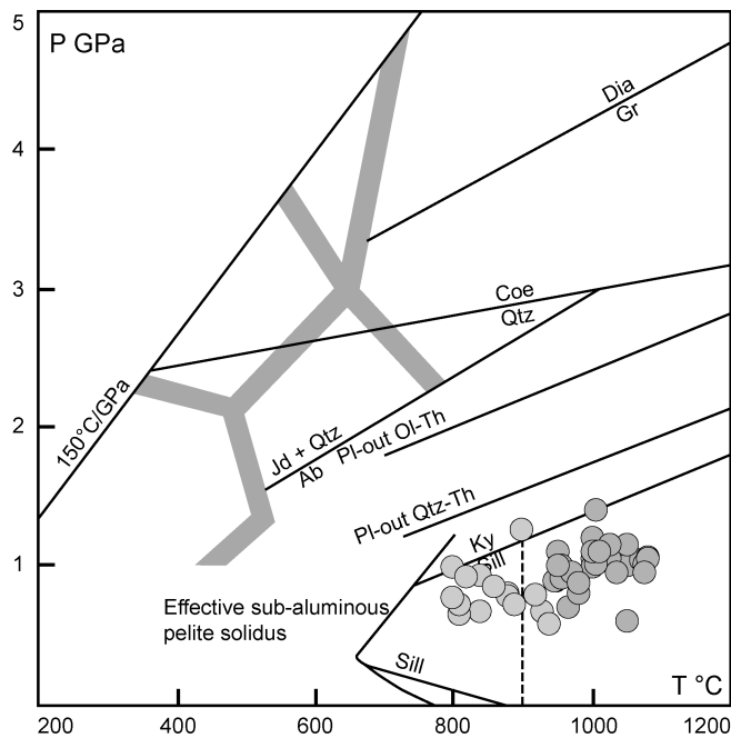
FIG. 4. Peak metamorphic P-T conditions of metamorphic belts: granulite-ultrahigh temperature (G-UHT) metamorphism (lighter grey symbols are granulite belts from Table 1 and darker grey symbols are UHT metamorphic belts from Table 2).
