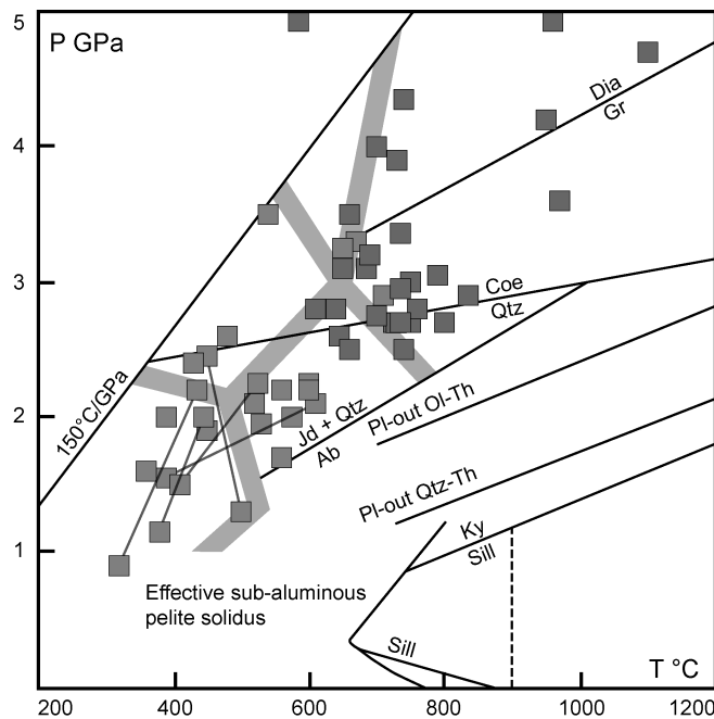
FIG. 6. Peak metamorphic P-T conditions of metamorphic belts: high pressure–ultrahigh pressure (HP–UHP) metamorphism (lighter grey symbols are lawsonite blueschists and eclogites from Table 4, lines join prograde and peak P-T conditions for some localities, and darker grey symbols are UHP metamorphic belts from Table 5).
