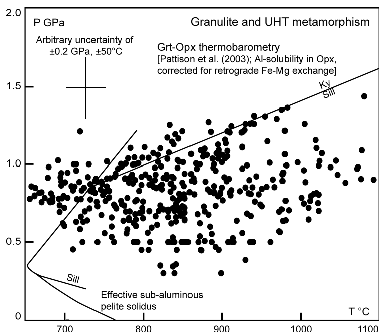
FIG. 2. Internally consistent thermobarometry of single rock samples of granulite and UHT metamorphism (Grt–Opx thermobarometry by Pattison et al., 2003 using Al-solubility in Opx corrected for retrograde Fe–Mg exchange).
