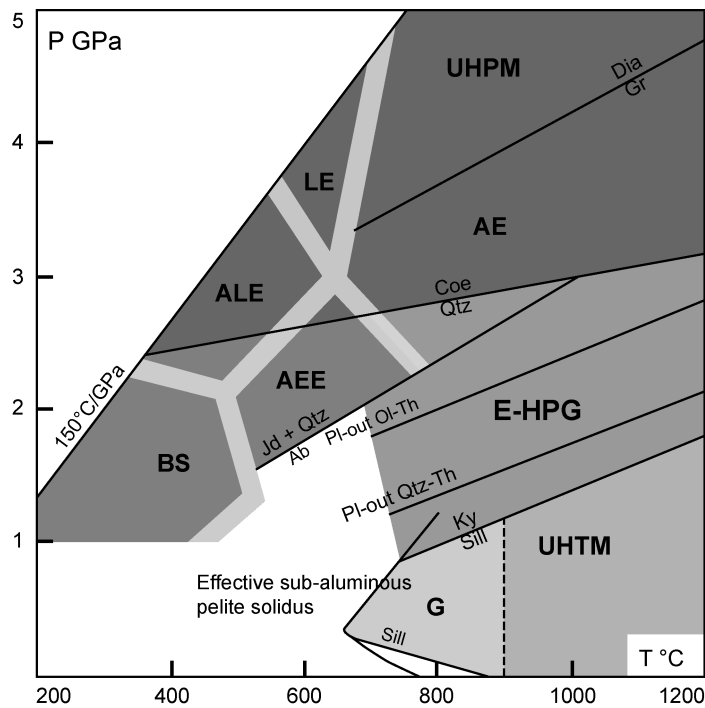
FIG. 1. P-T diagram illustrating conditions of selected metamorphic facies and P-T ranges of different types of metamorphism. HP-UHP metamorphism includes the following: BS = blueschist; AEE = amphibole-epidote eclogite facies; ALE = amphibole-lawsonite eclogite facies; LE = lawsonite-eclogite facies; AE = amphibole-eclogite facies; UHPM = ultrahigh-pressure metamorphism; E-HPG = eclogite-high-pressure granulite metamorphism; G = granulite facies, whereas UHTM = ultrahigh-temperature metamorphic part of the granulite facies.
