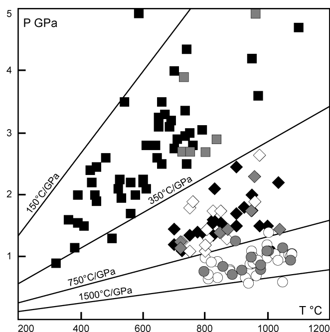
FIG. 7. Metamorphic patterns by belt in relation to thermal gradients and age (filled symbols are belts where peak P-T conditions were recorded at < 488 Ma, grey symbols are belts where peak P-T conditions were recorded at < 850 but > 488 Ma, and open symbols are belts where peak P-T conditions were recorded at > 850 Ma).
