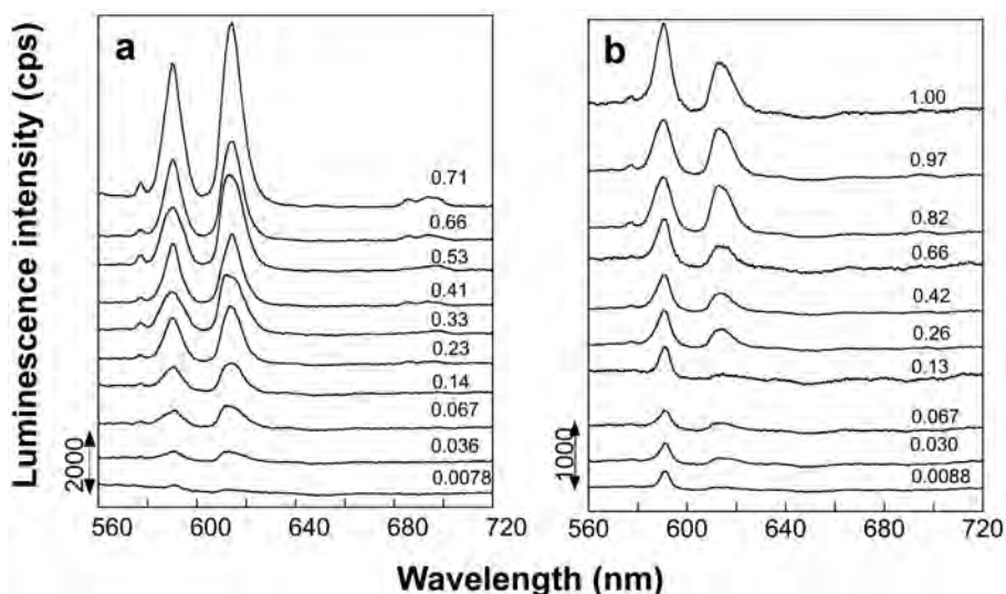
Figure 3. Luminescence spectra of reaction products of \text{EuCl}_3 with (a) Sumecton SA and (b) \text{Na}^+ -TSM. The numbers along the right side of each figure designate the amount of \text{Eu}^{3+} (meq/g of clay).
