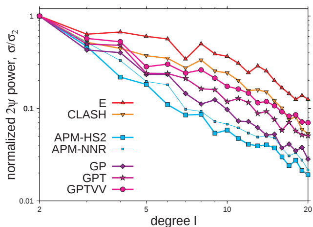
Figure 3. 2\Psi power normalized by \sigma_2 , \sigma_1/\sigma_2 , for seismological and geodynamic models at 50 s on a log – log plot; see Table 1 for abbreviations.
