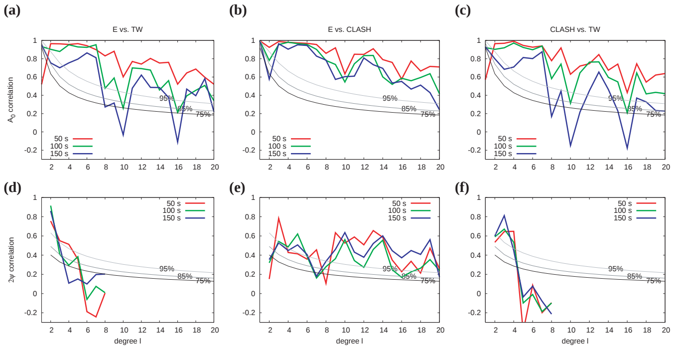
Figure 4. Correlation as a function of degree r_l , eq. (12), for isotropic, A_0 , (a, b and c) and 2\Psi anisotropic (d, e and f) structure at periods between 50 and 150 s for the seismological models. We compare E and TW (a and d), E and CLASH (b and e), and CLASH and TW (c and f). Correlation plots are shown only up to L = 8 for 2\Psi from TW because of the effectively limited resolution due to damping choices. Confidence levels at 75, 85 and 95 per cent are plotted following Student's t distribution, eq. (13). Total correlation values for L = 8 are listed in Table 3 and displayed in Fig. 5.
