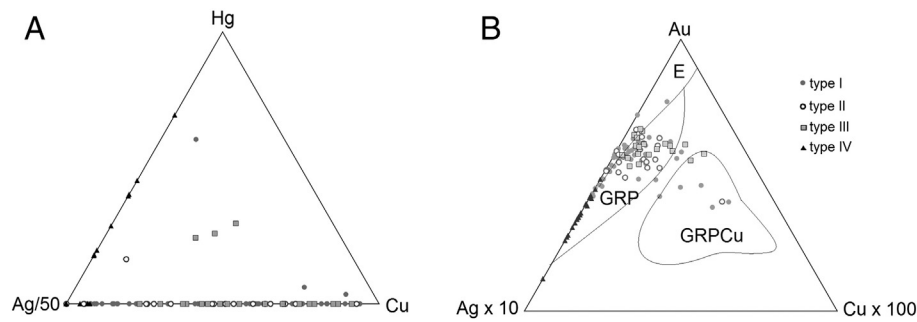
Fig. 9. The analysis of the chemical composition of Vagran cluster placer gold alloys from the cores of the grains, classified: A – in the terms of Ag/50–Cu–Hg; B – in the terms of Au–Ag \times 10–Cu \times 100. The compositional fields of gold grains according to Townley et al. (2003) and Chapman et al. (2011) and plotted on B: E – for epithermal deposits, GRP – for gold rich porphyry deposits, GRPCu – for gold-rich porphyry copper deposits.
