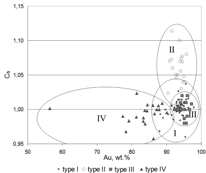
Fig. 10. Au content in the core of grains (wt.%) vs coefficient of heterogeneity ( C_h ) plot for Vagran cluster placer gold. The diagram distinguishes the types of gold grains both by primary hypogenic characteristics and supergenic features.
