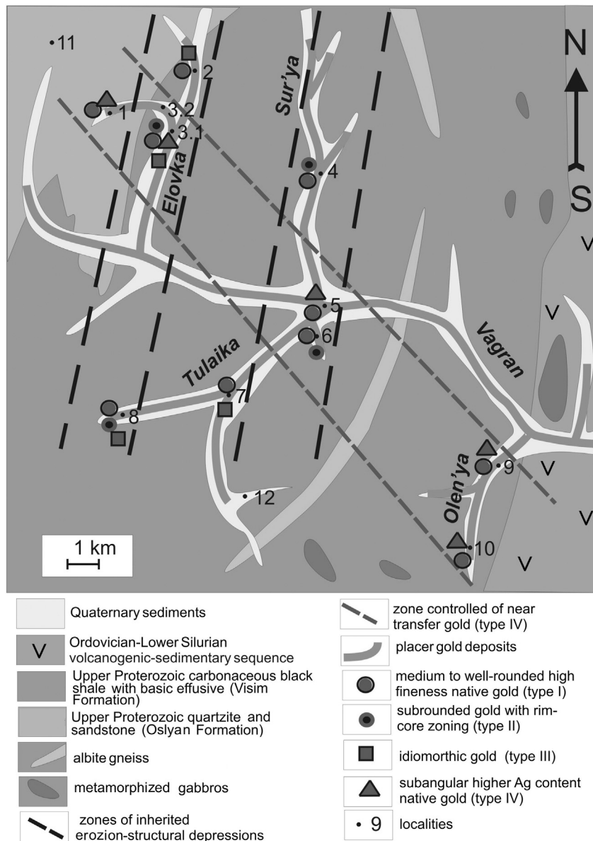
Fig. 2. Geological map of Vagran gold cluster with placer gold metallogeny (based on the Geological report, 1967) with data from current research that demonstrates the distribution of various types of the placer native gold over the territory of the cluster. The zone of NW-SE trend indicates the location of the gold with short transport indicators.
