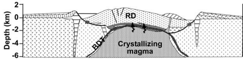
Figure 1. Conceptual model of a caldera [after Lipman, 1984] which includes the boundary faults and a resurgent dome (RD). The brittle-ductile transition (BDT) coincides with a transition from lithostatic (below) to hydrostatic (above) pressure distribution (following Fournier [1999]). The arrows represent fluid derived from magma crystallization, being injected into the base of the hydrothermal system.
