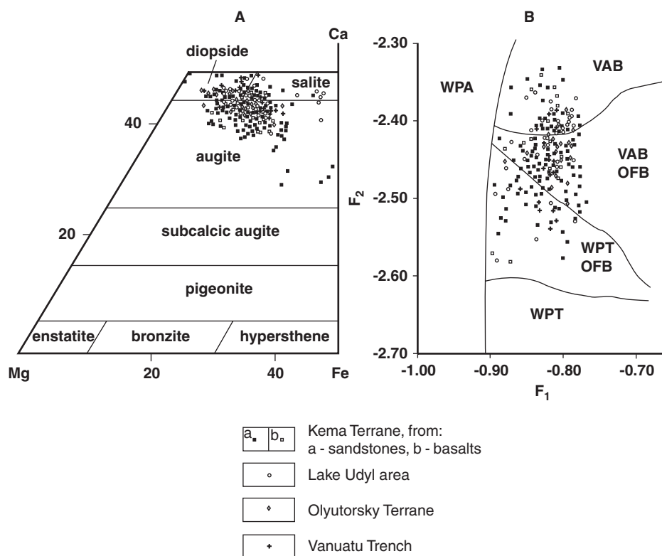
Fig. 4. (A): Comparative diagram showing composition of clinopyroxenes from basalts and sandstones; (B): Discriminant diagram for basalt-hosted clinopyroxenes from different geodynamic settings (after Nisbet and Pearce, 1977). VAB: volcanic arc basalts; OFB: ocean-floor basalts; WPT: within-plate tholeiitic basalts; WPA: within-plate alkaline basalts. F_1 = -0.012 \times \text{SiO}_2 - 0.0807 \times \text{TiO}_2 + 0.0026 \times \text{Al}_2\text{O}_3 - 0.0012 \times \text{FeO} - 0.0026 \times \text{MnO} + 0.0087 \times \text{MgO} - 0.0128 \times \text{CaO} - 0.0419 \times \text{Na}_2\text{O} ; F_2 = -0.0496 \times \text{SiO}_2 - 0.0818 \times \text{TiO}_2 - 0.02126 \times \text{Al}_2\text{O}_3 - 0.0041 \times \text{FeO} - 0.1435 \times \text{MnO} - 0.0029 \times \text{MgO} - 0.0085 \times \text{CaO} + 0.0160 \times \text{Na}_2\text{O} .
