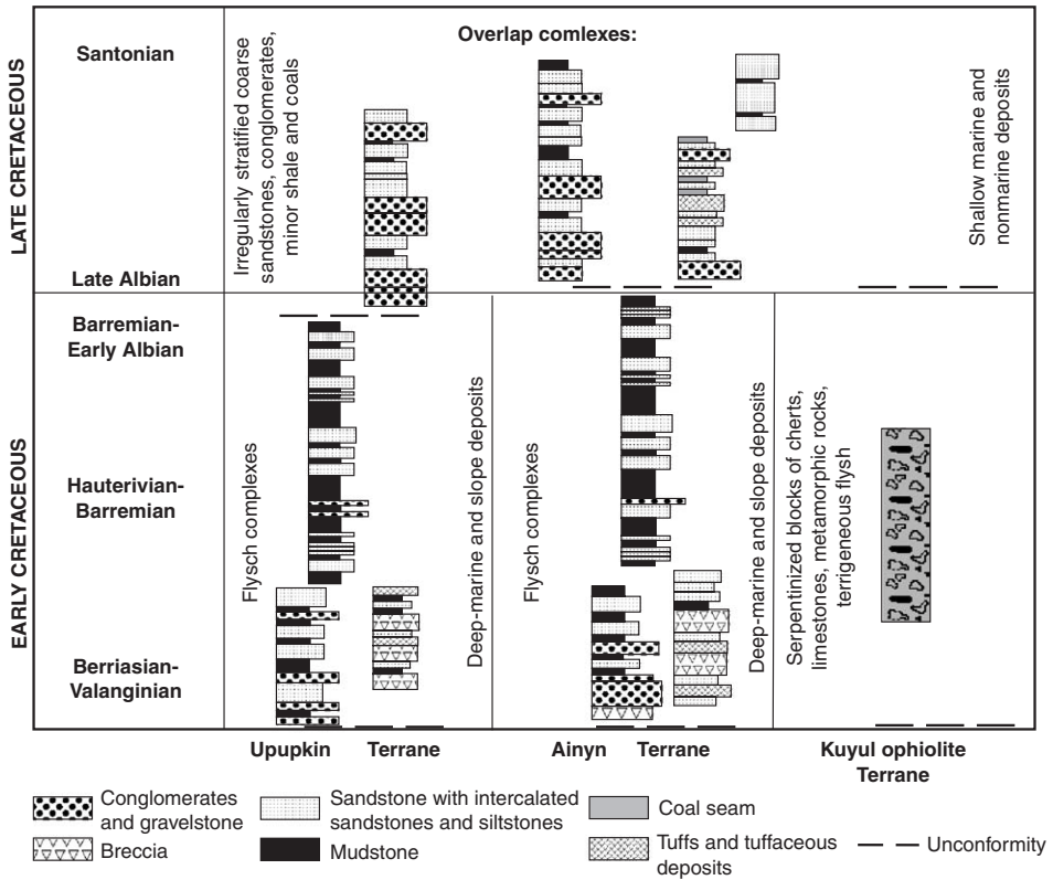
Fig. 14. Generalised lithostratigraphy of the Upupkin, Ainyin, and Kuyul ophiolite terranes.
