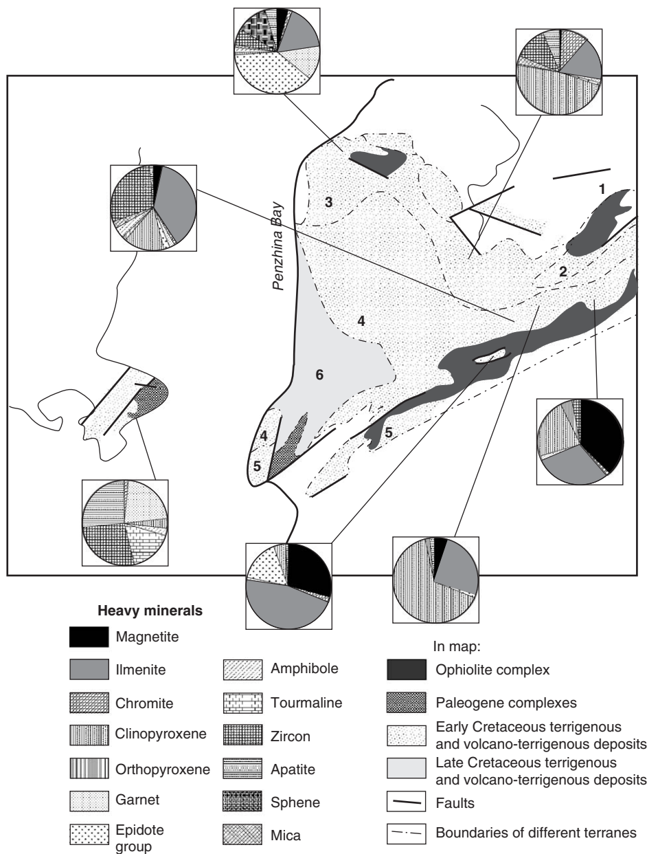
Fig. 15. Average heavy mineral associations in the Berriasian-Valanginian deposits. Numbers in map are the main terranes 1: Kharitonia; 2: Ganychalan; 3: Upupkin; 4: Ainyn; 5: Kuyul ophiolite; 6: Albian-Upper Cretaceous overlap complexes.
