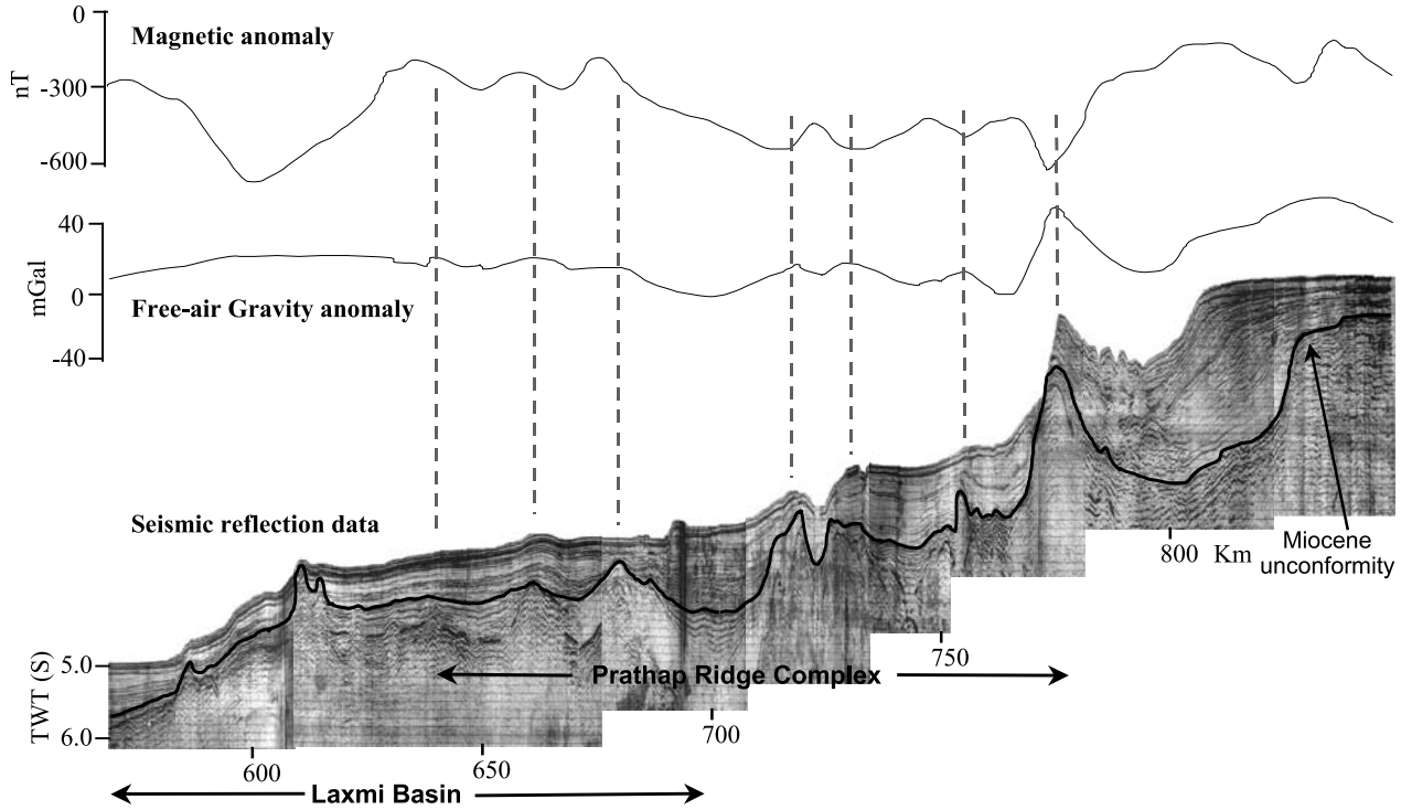
Figure 7a. Seismic reflection profile (eastern part of RE-11) across the continental margin. Prathap Ridge Complex and part of the Laxmi Basin are integrated with gravity and magnetic anomaly data. Miocene sedimentary boundary is shown with a solid undulating line in the sediment column. Volcanic intrusive structures coincide with the magnetic anomalies (shown by solid track).
