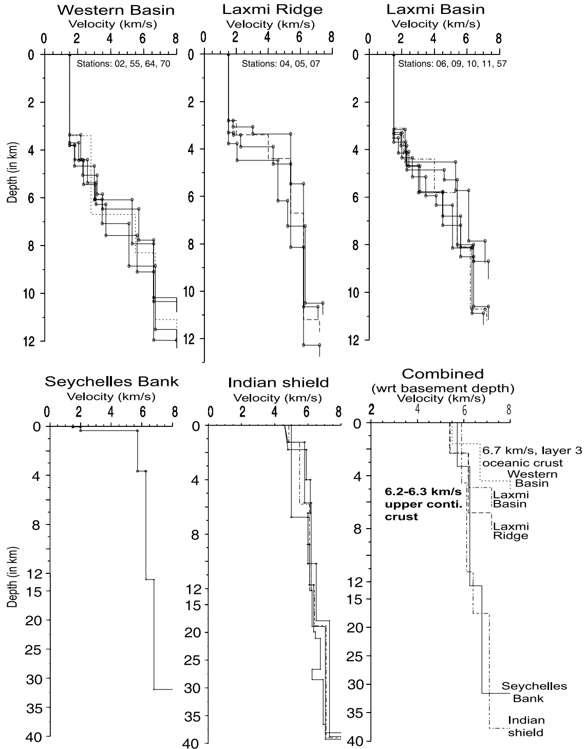
Figure 10. Velocity-depth plots from sonobuoy stations of the Western Basin, Laxmi Ridge, Laxmi Basin, Seychelles Bank, and western Indian shield [Naini and Talwani, 1983; Davies and Francis, 1964; Matthews and Davies, 1966; Reddy et al., 1999]. Noncontinuous lines in graphs of Western Basin, Laxmi Ridge, Laxmi Basin, and Indian shield represent the average crustal velocities and thicknesses. In bottom right, crustal columns and velocities of all the regions are stacked with respect to the basement. The 6.7 km/s velocity layer (oceanic layer 3) of the Western Basin is absent beneath the Laxmi Ridge and Laxmi Basin. The anomalous velocity layer 7.0 to 7.4 km/s is noticed in the lower crust of the Laxmi Ridge and Laxmi Basin.
