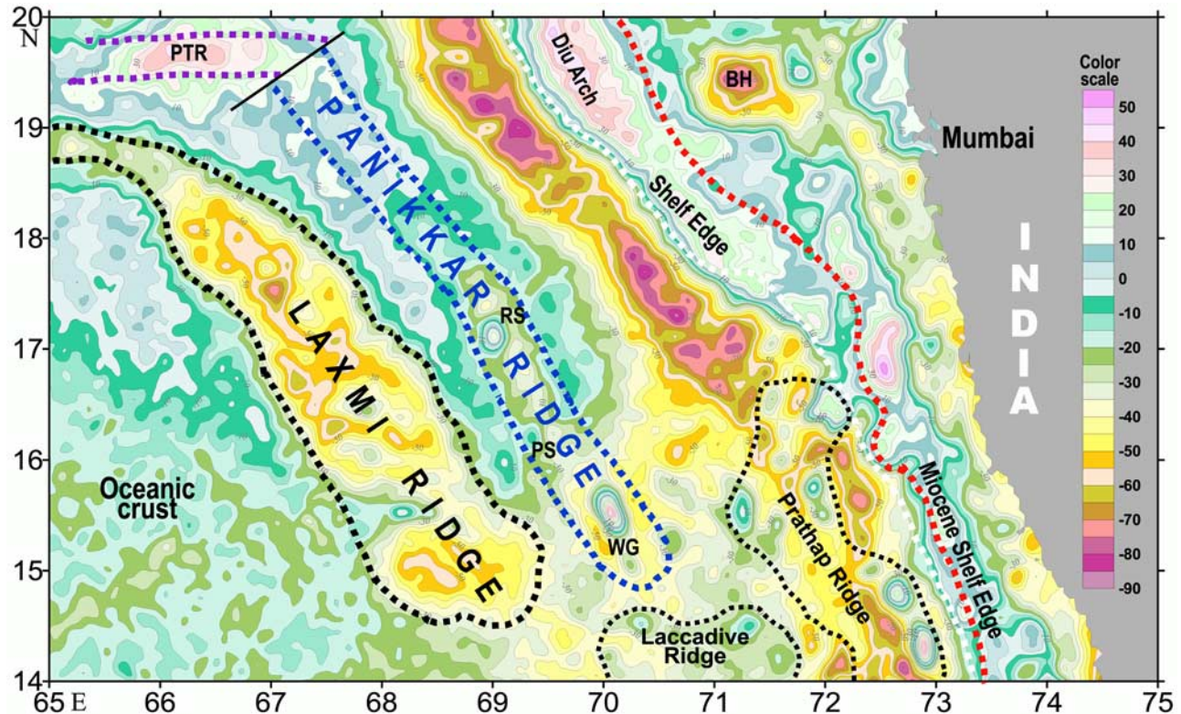
Figure 9. Map of satellite free-air gravity anomalies [Sandwell and Smith, 1997] and interpreted geomorphic features. Features are outlined by square-dotted lines and are labeled WG, Wadia Guyot; RS and PS, Raman and Panikkar seamounts, respectively; PTR, Palitana Ridge; PR, Panikkar Ridge; and BH, Bombay High structure.
