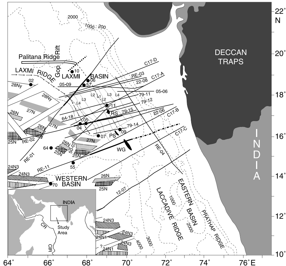
Figure 1. General bathymetry of the Laxmi Basin and adjoining regions. Depths are in meters. Lines with labeling show the geophysical profiles. Magnetic isochrons 28Ny-24N1 are shown on west of the Laxmi Ridge [Chaubey et al. , 1998]. Locations of seismic sonobuoy stations are marked by solid circles. L1–L4 represent magnetic lineations identified by Bhattacharya et al. [1994a]. Solid dashed line along L1, WG, PS, and RS represent Panikkar Ridge, Wadia Guyot, Panikkar seamount, and Raman seamount, respectively. Arrows circled by dashed line show axis and boundaries of the Laxmi Ridge. Seismic sections of solid tracks along the profiles RE-01, RE-02, and RE-11 are shown in Figure 3. Seismic, gravity, and magnetic data along the solid track and dash-dotted track on profile RE-11 are shown in Figures 7a and 7b, respectively.
