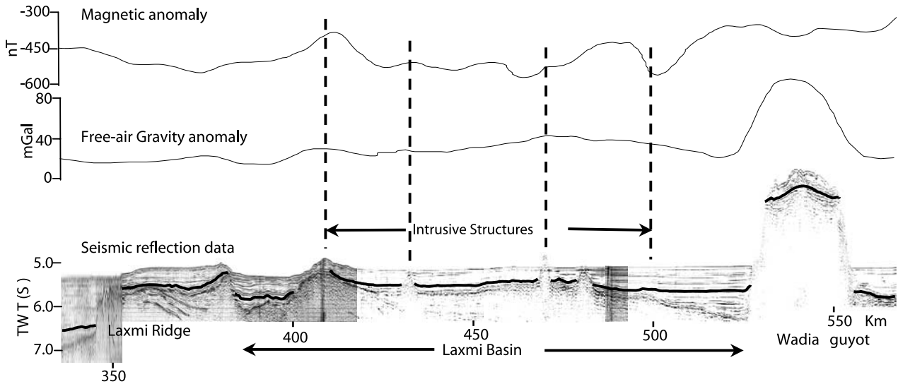
Figure 7b. Seismic reflection profile (central part of RE-11) across the Wadia Guyot. Part of the Laxmi Basin and Laxmi Ridge is integrated with gravity and magnetic anomaly data. Miocene sedimentary boundary is shown with a solid undulating line in the sediment column. Volcanic intrusive structures coincide with the magnetic anomalies (shown by dash-dotted track).
