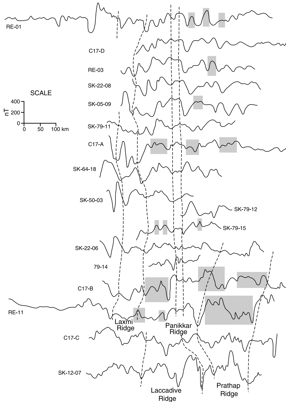
Figure 6. Magnetic profiles collected on board various research vessels. ORV Sagar Kanya (SK 05, 12, 22, 50, 64, and 79), MV Anweshak (RE lines), and R/V Conrad (C1707) are stacked with reference to the Panikkar Ridge. Geometric proton Precession magnetometer was used on board the research vessels ( Sagar Kanya and Anweshak ) to record the total field magnetic data, which subsequently reduced to anomaly by subtracting the International Geomagnetic Reference Field values. Dashed lines show correlated anomalies of the Prathap, Laccadive, Panikkar, and Laxmi ridges. The anomalies that are seen associated with volcanic structures on the seismic sections are shaded.
