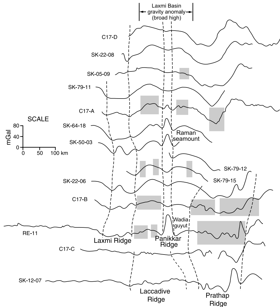
Figure 5. Gravity profiles collected on various cruises of research vessels. ORV Sagar Kanya (SK 05, 12, 22, 50, 64 and 79), MV Anweshak (RE lines), and R/V Conrad (C17A-D) are stacked with reference to the Panikkar Ridge. KSS-30 Bodenseewerk and Lacoste-Romberg gravimeters with reference base system IGSN-71 were used on board the research vessels Sagar Kanya and Anweshak , respectively, to record the gravity data. Free-air gravity anomalies were calculated by applying the Eötvös correction and normal gravity (with reference to ellipsoid GRS 67) at the observation positions. Dashed lines show correlated anomalies of the Prathap, Laccadive, Panikkar, and Laxmi ridges. The anomalies that are seen associated with volcanic structures on the seismic sections are shaded.
