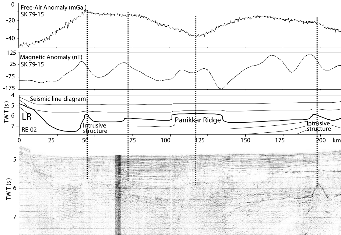
Figure 8. Seismic reflection record and its interpreted crustal section of profile RE-02 and free-air gravity and magnetic anomalies of nearly coincident profile SK 79-15. Both the profiles were acquired very closely in the Laxmi Basin. Dotted lines show axis of Panikkar Ridge and volcanic structures.
