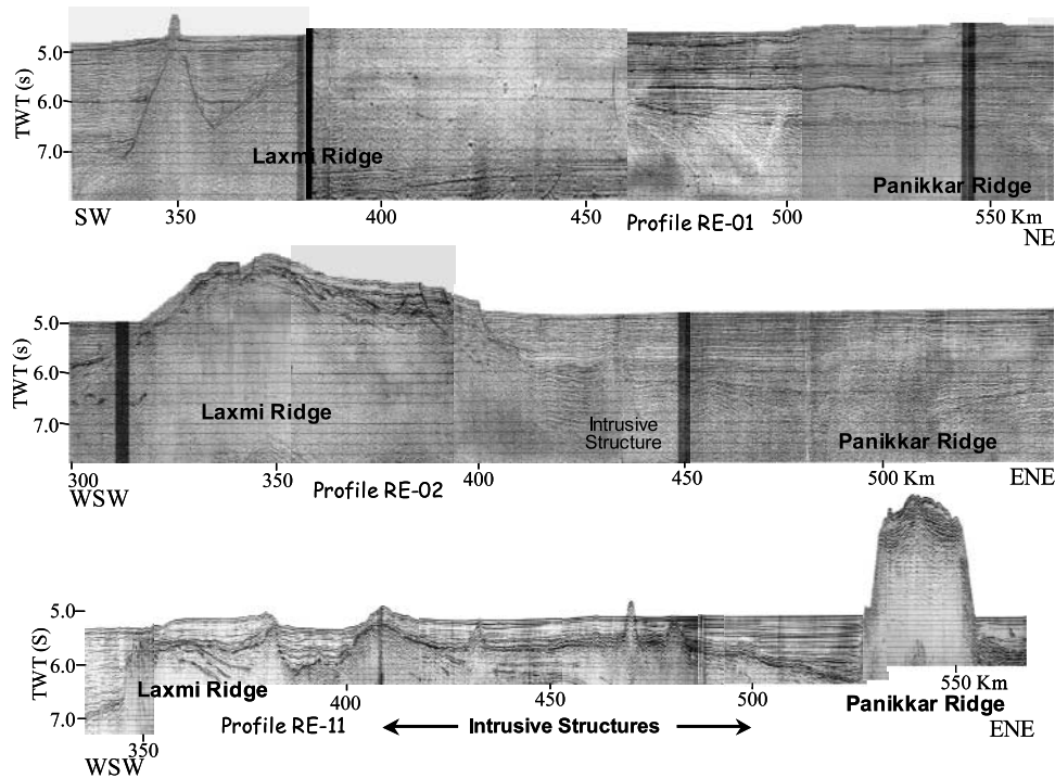
Figure 3. Seismic reflection images of the Laxmi and Panikkar ridges along RE-01, RE-02, and RE-11 profiles. Locations of the sections are shown with a solid line along the profiles in Figure 1.
