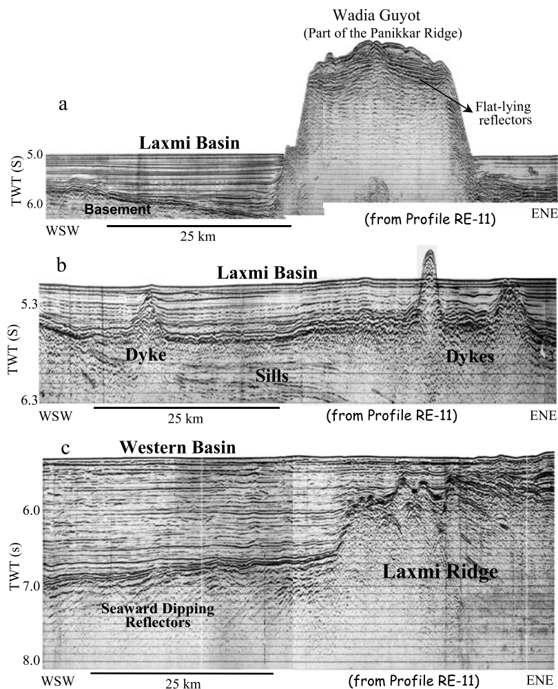
Figure 4. Seismic reflection sections (profile RE-11) of (a) basement topography and stratified sediments of the Wadia Guyot, (b) dikes and sills in the Laxmi Basin, and (c) series of intrabasement seaward dipping reflectors on west of the Laxmi Ridge. The SDRs deepen to the west, and their feather edges occur at shallow depth in the east.
