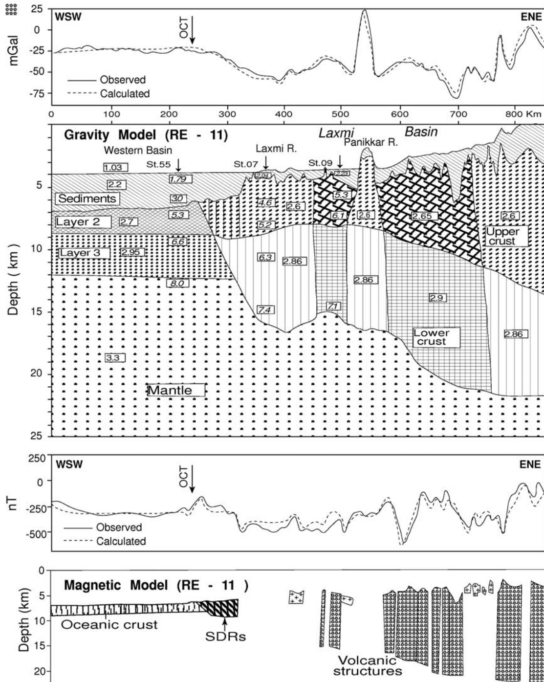
Figure 11. Modeled crust structure across the continental shelf, Laxmi Basin, Panikkar Ridge, Laxmi Ridge, and eastern Arabian Sea from free-air gravity and magnetic anomalies. The Laxmi Basin basically consists of stretched continental crust, while the crust adjacent to the Panikkar Ridge in the basin is intermixed with the Deccan volcanic rocks. Magnetic anomalies are modeled with intrusive structures caused by the Deccan volcanism. Seaward dipping reflectors are considered for modeling the magnetic anomaly on west of the Laxmi Ridge. Parameters used in anomaly computations are densities 1.03–3.3 g/cm 3 , total magnetic field 40400 nT, and remanent magnetization 1.0–4.0 A/m. For reversal magnetic bodies (shown with plus sign), inclination is +50° and declination is +130°. For normal magnetic bodies (shown with open star), inclination is –50° and declination is –40°. Long-range sonobuoy (stations 55, 07 and 09, close to profile RE-11) velocity results are projected onto the crustal model. The values below the stations represent the velocities in km/s.
