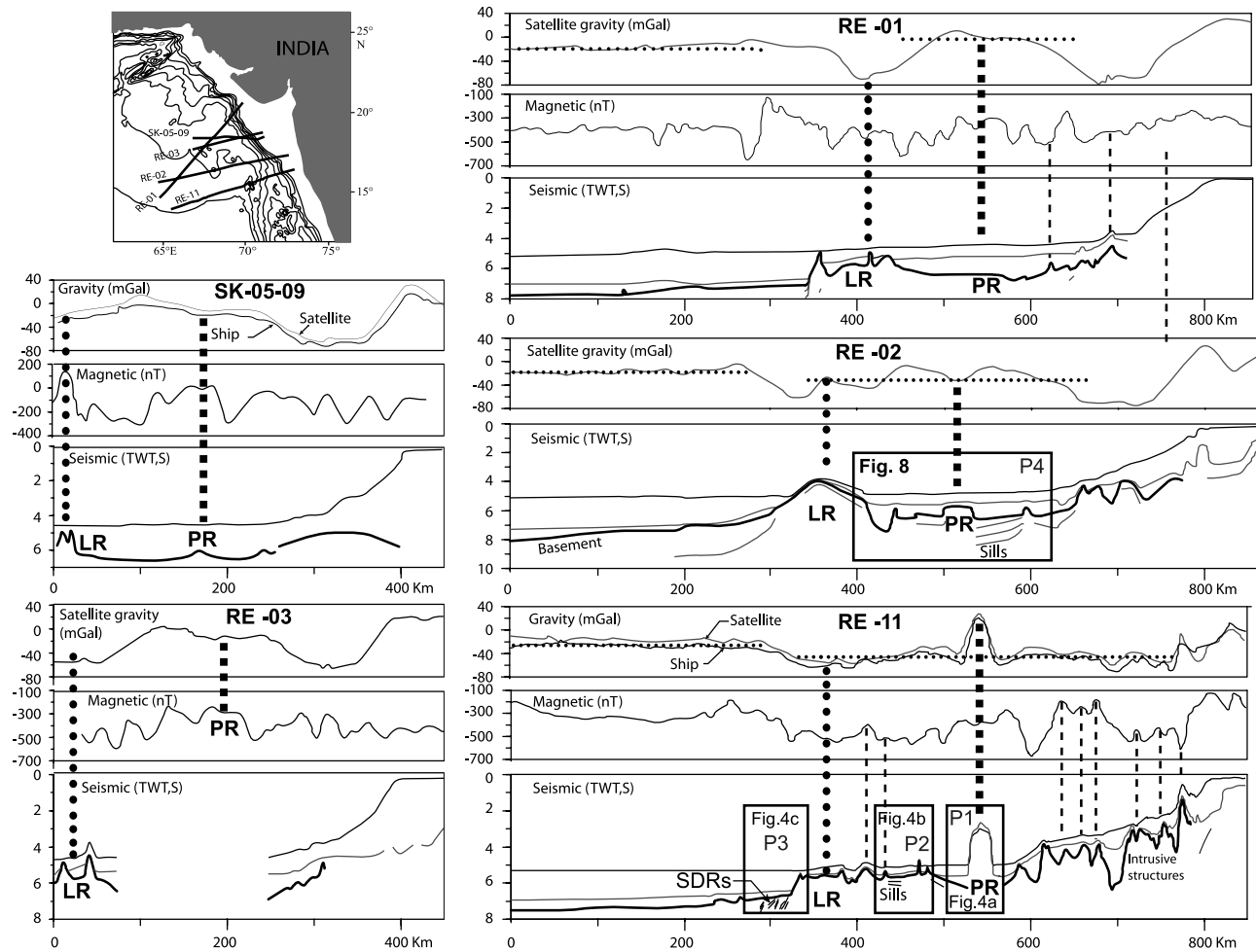
Figure 2. Stacked regional geophysical profiles of interpreted multichannel seismic reflection, free-air gravity, and magnetic anomalies. Locations of profiles are shown in top left corner. Profiles RE-01, RE-02, RE-03, RE-04, and RE-11 were acquired using Digital Field System (DFS) IV instrument on board MV Anveshak with 48-channel seismic streamer, using Bolt-type air gun array with a total capacity of 10 L. A DFS V instrument system, 24-channel seismic streamer and D-type array of seven air guns with a total capacity of 7.98 L were used aboard ORV Sagar Kanya for acquisition of data on profiles SK 05-06 and 05-09. P1, P2, P3, and P4 are seismic sections shown in Figures 4 and 8, respectively. PR and LR represent Panikkar and Laxmi ridges, respectively. Vertical dotted lines show correlations between volcanic intrusive structures and magnetic anomalies.
