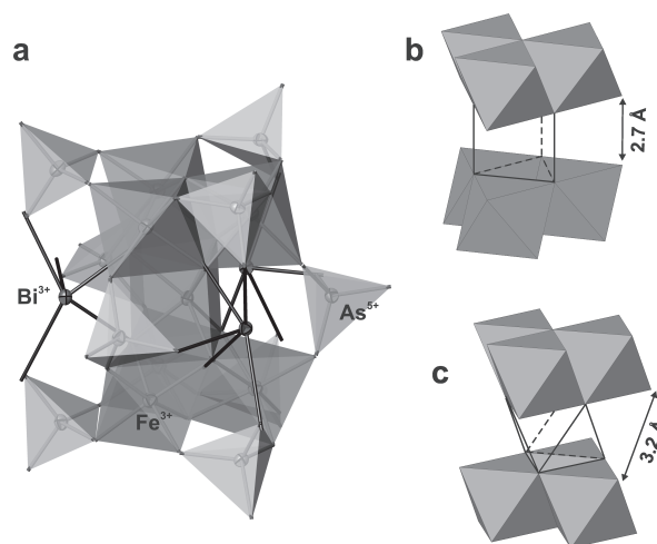
FIGURE 4. The [\text{Bi}_3\text{Fe}_7\text{O}_6(\text{OH})_2(\text{AsO}_4)_9]^{11-} nanocluster in the structure of bouazzerite (a) and two schemes used to explain trigonal prismatic coordination of the Fe5 site (b, c). See text for details.
