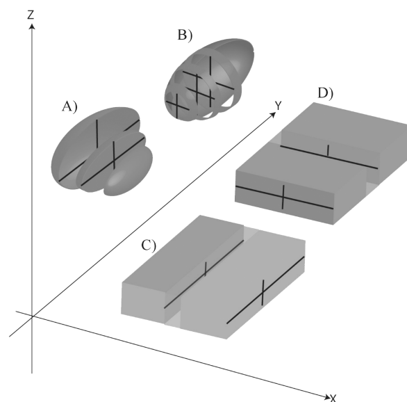
Fig. 2. A clast morphology diagram that demonstrates how observed clast shape is controlled by location of intersection plane and primary clast shape, and how apparent clast size can be impacted by position of intersection plane relative to clast centroid. Clast distribution pattern is affected by primary shape of clast and by distribution of clasts. A fabric can be produced by a series of elongate clasts, or a preferred alignment of a number of equant clasts. a) Ellipsoidal clast with intersection planes parallel to XZ. b) Ellipsoidal clast with intersection planes parallel to YZ. Both (a) and (b) show how the observed size of a spherical or ellipsoidal clast will vary depending on the position of the intersection plane relative to the centre of the spherical clast. c) Cubic clast with intersection planes parallel to YZ. d) Cubic clast with intersection planes parallel to XZ. Both (c) and (d) show how for the sphere and the cube the observed clast shape is totally independent of view direction.
