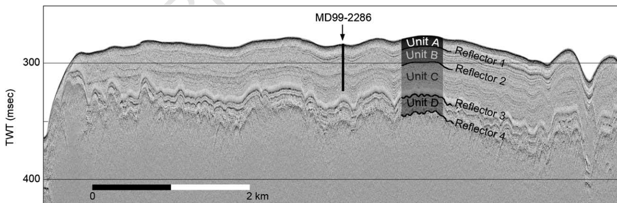
Figure 3 Chirp sonar profile from the MD99-2286 coring site. The seismic units A–D and reflectors 1–4, defined by Gyllencreutz et al. (1995), are indicated in the profile. The penetration depth of MD99-2286 (indicated with a black vertical line) was estimated from correlation of MST-measured GRA-density and the chirp sonar record at the coring site (Gyllencreutz et al. , 2005). TWT, two-way travel time
