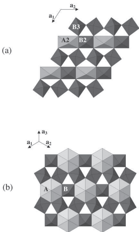
FIGURE 1. (a) M layer (at z \sim 1/6 ) in the structure of ingersonite (projection down [001]); (b) M layer in the structure of pyrochlore (projection down [111]).
