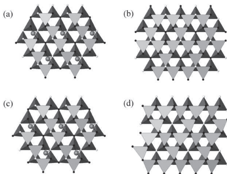
FIGURE 4. Arrangements of anion-centered X(A,B) 4 tetrahedra in ingerssonite (a), pyrochlore-type structure (b), weberite-type polytypes (c), zirconolite-type polytypes (d). Black and white small circles represent A and B cations, respectively. Gray circles represent the three-coordinated oxygen atoms asymmetrically located in octahedral interstices.
