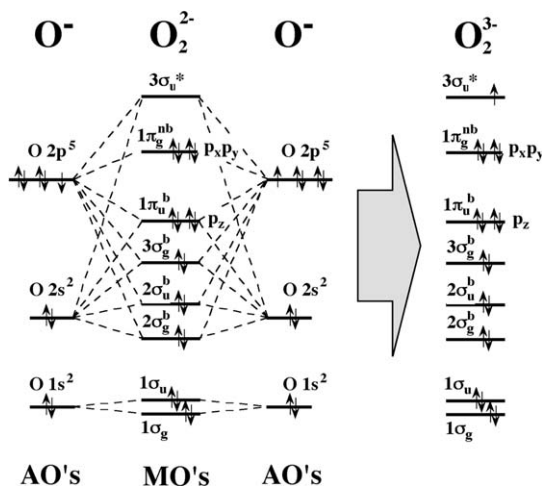
Fig. 3a. Schematic representation of the energy levels of the bonding, non-bonding and antibonding molecular orbitals in the peroxy anion, O_2^{2-} and O^- using Molecular Orbital concepts (see text).
