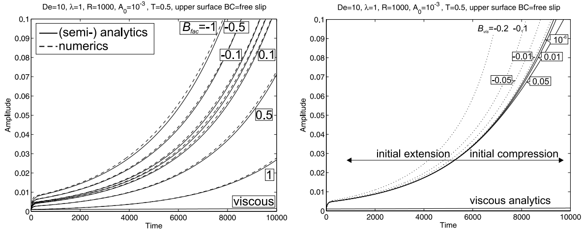
Figure 6. (a) Effect of a gravity-driven pre-stress state on the growth of the instability. Both numerical and analytical solutions are shown. The viscous case ( De \ll 1 ) is plotted for comparison. (b) Effect of initial pure-shear compressional state of the system for a two-layer case in which elasticity is important ( De = 10 ). All other parameters as in Fig. 4; only numerical solutions are presented. An initial extensional stress state increases the growth rate, whereas an initial compressional stress state decreases the growth rate. Compressional stress states beyond 0.05 resulted in buckling-type instabilities.
