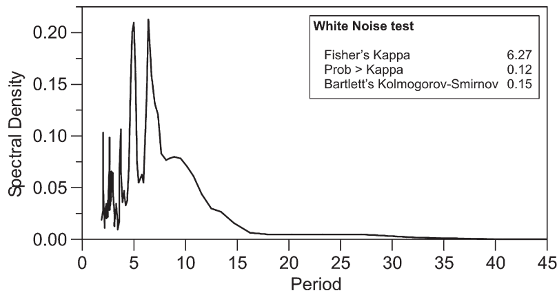
Figure 4 Spectral density analyses of the 163-yr masterchronology. The time series shows significant periodic components ( P < 0.05 ). Note peaks between 5 and 7 years
