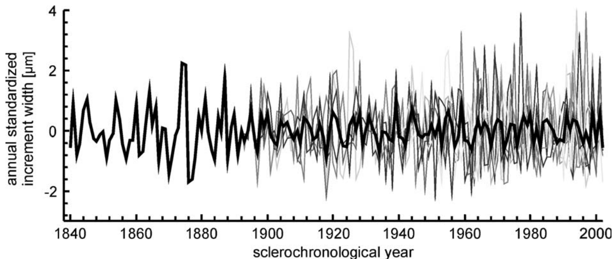
Figure 3 163-yr masterchronology (black line) of A. islandica . Grey lines indicate the eight standardized time index series the masterchronology is based on. Note that between 1840 and 1896 only one shell was available for the masterchronology, therefore amplitudes are higher than between 1896 and 2001
