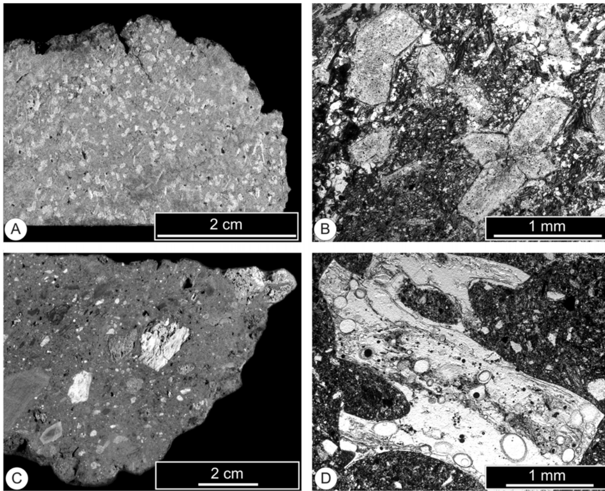
Fig. 5. Impact-related lithologies present at localities south of the unpaved road between Nyameani and Nkowinkwanta (~2.7 km off the northern shore of Lake Bosumtwi, Ghana) (cf. Fig. 1). a, b) Two mica schists with up to 20 vol% sericite pseudomorphs after twinned staurolite crystals. Sample BOT 6. c, d) Glass-rich suevite with a clast population comprising schists, slates rich in organic material, whole-rock melt glass, and mineral fragments, among those quartz melt glass and diaplectic quartz glass with coesite. Sample BOT 12. d) Schlieren-rich melt glass fragment with numerous vesicles/bubbles lined with clay minerals in a clastic matrix consisting of rock fragments and clasts of tectosilicates, chlorite, biotite, and sericite. (a) and (c) are hand-specimens; (b) and (d) are micrographs // nicols.
