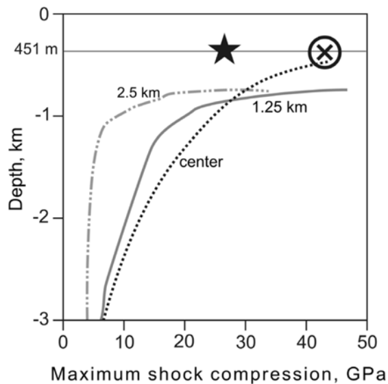
Fig. 15. Depth-shock pressure graph for three modeled drilling locations at Lake Bosumtwi, at the crater center (dotted), 1.25 (line), and 2.5 km (chain dotted) off the center. The horizontal line corresponds to the final depth of well LB-08A, the star to the maximum shock pressure derived from petrographic analysis of the target rocks, the cross to the maximum pressure derived from the model (i.e., <45 GPa). Modified after Artemieva et al. (2004).
