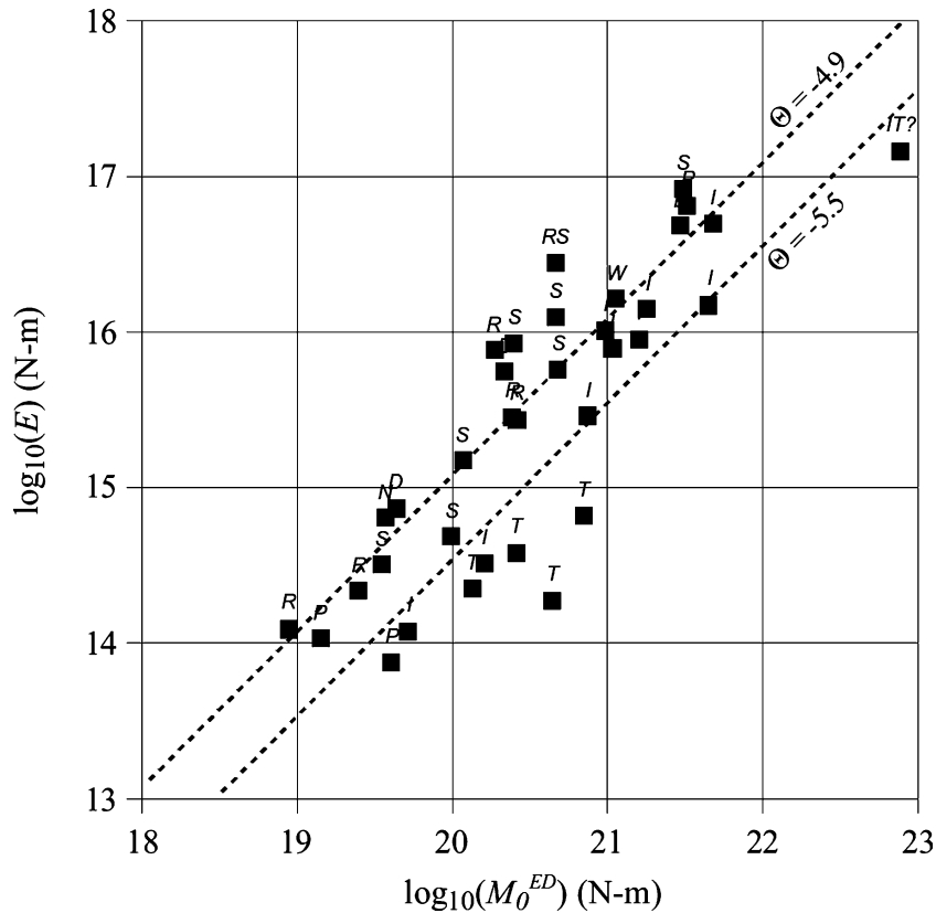
Figure 7. Estimated radiated energy E compared to the moment M_0^{ED} from this study. Lines of constant \Theta are shown for \Theta = -4.9 , the expected value for all earthquakes, and \Theta = -5.5 , below which indicates a possible tsunami earthquake. Events are labelled by their source types (see Table 1).
