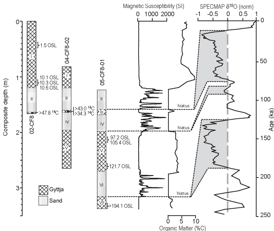
Figure 2. Stratigraphic context of ^{14}\text{C} and optically stimulated luminescence (OSL) ages, shown in thousands of years B.P. ^{14}\text{C} ages from unit III are given in Table DR1, and OSL ages are given in Table DR2 (see footnote 1). Composite magnetic susceptibility (MS) and organic matter (OM) content were generated by splicing MS and OM content from individual cores using unit contacts as tie points. The global ice volume proxy, normalized oceanic \delta^{18}\text{O} , is from Martinson et al. (1987).
