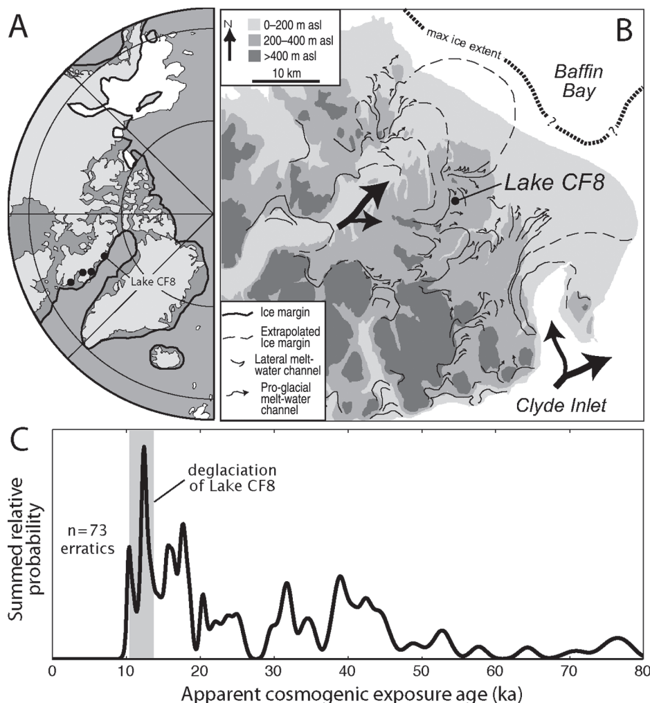
Figure 1. Location maps. A: Sites where pre-Holocene organic sediments have been recovered (black dots) within glaciated North America (black line), including Lake CF8. B: Lake CF8 and surrounding glacial-geologic features on the Clyde foreland. Large arrows indicate former flow directions of the Laurentide Ice Sheet, which deposited erratics across the landscape (asl—above sea level). C: Summed relative probability distribution of 73 erratics from relict landscape near Lake CF8 dated by ^{10}\text{Be} and ^{26}\text{Al} exposure dating (from Briner et al., 2005) reveals several modes, the youngest of which represents last deglaciation. Multiple modes illustrate prevalence of cosmogenic radionuclide inheritance in terrains formerly covered by cold-based ice.
