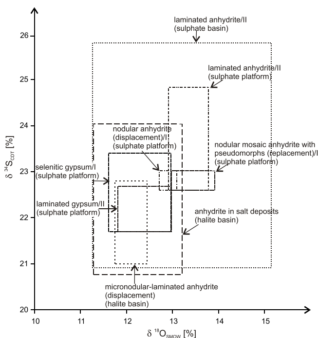
Fig. 5. Oxygen and sulphur isotope composition of Badenian sulphates (gypsum and anhydrite) in the Carpathian Foredeep (based on data from: Bukowski and Szaran, 1997; Kasprzyk, 1997, 2003; Peryt et al. , 1998; Cendón et al. , 2004)
