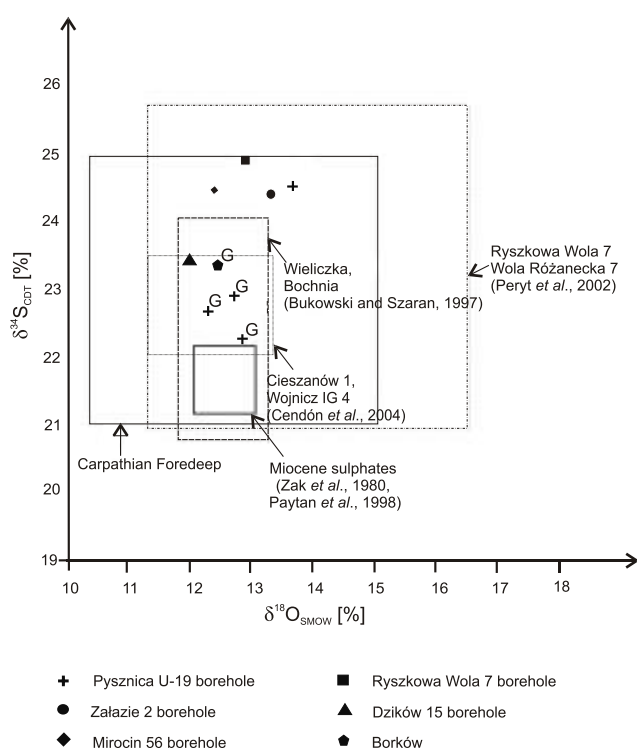
Fig. 6. Plot of \delta^{34}\text{S} and \delta^{18}\text{O} values in studied gypsum and anhydrite samples
