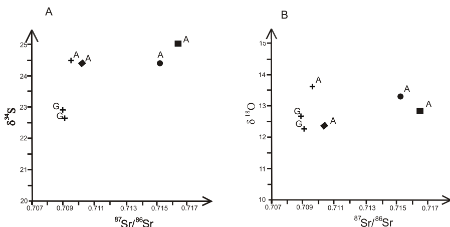
Fig. 7. Relationship between ^{87}\text{Sr}/^{86}\text{Sr} and \delta^{34}\text{S} (A) and ^{87}\text{Sr}/^{86}\text{Sr} and \delta^{18}\text{O} (B) of sulphate deposits: gypsum (G) and anhydrite (A)
