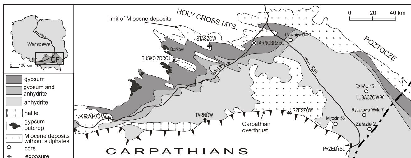
Fig. 1. Distribution of Badenian sulphate facies in the Carpathian Foredeep of Poland
