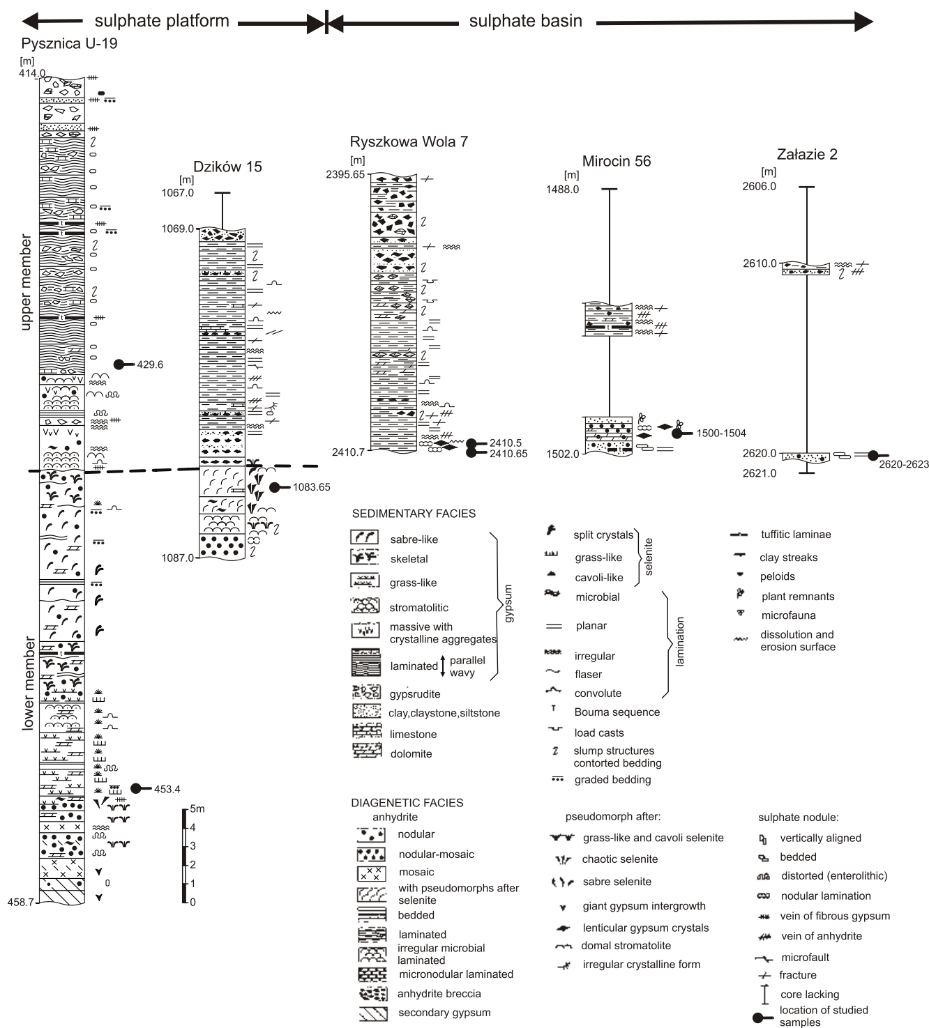
Fig. 2. Badenian sulphate successions representative of various settings, and locations of studied samples
