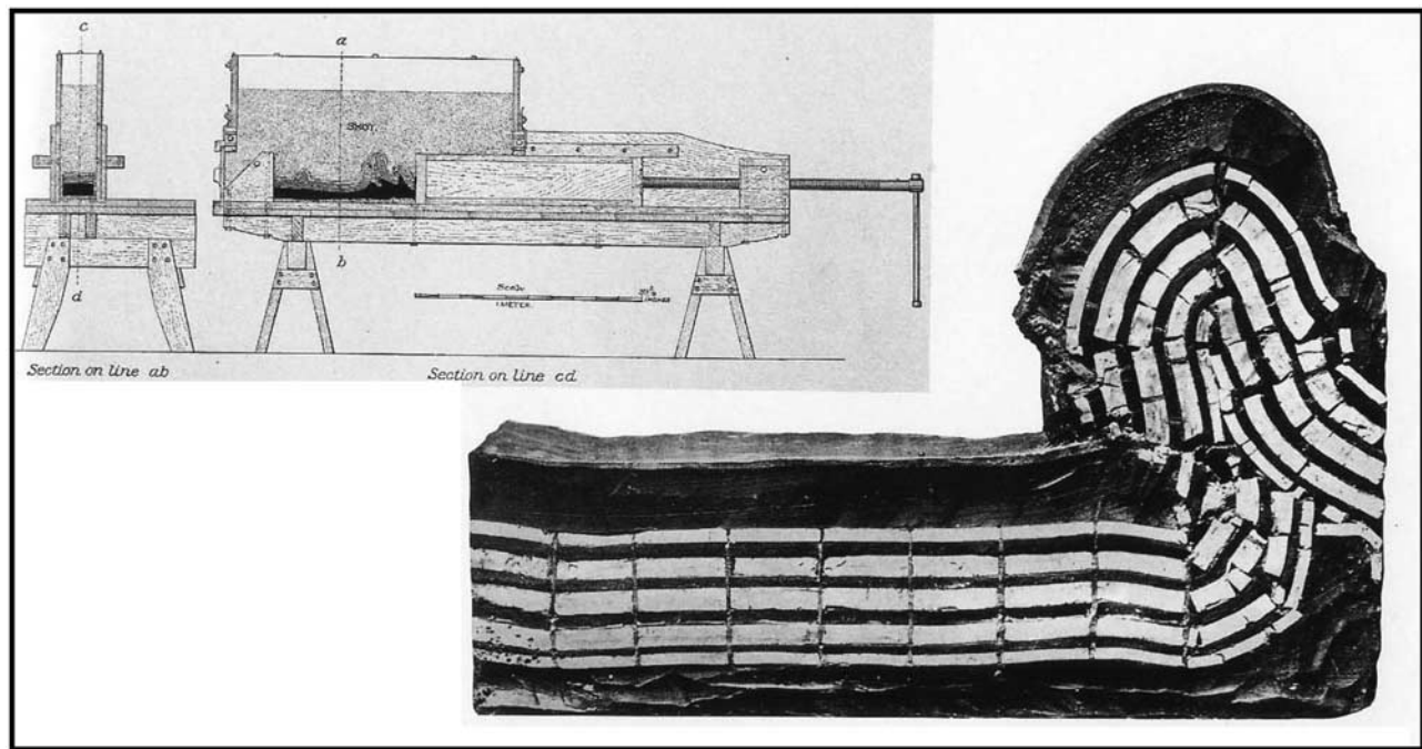
Figure 1. Sketch of the apparatus constructed by Willis [1891] to investigate folding mechanisms. The layers, representing geological strata, are made out of wax, and the model is overlain with lead sheets to qualitatively take into account the effect of gravity.
