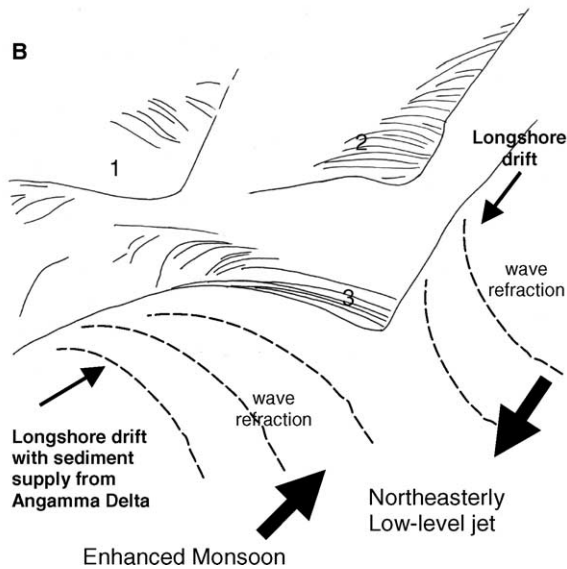
Figure 5 Cusped forelands to the east of the Angamma delta. (A) Landsat Band 4 image of the cusped forelands. (B) Line drawing interpretation of the Landsat image showing reconstruction of waves driven by southwesterly (Monsoon) and northeasterly (Harmatan) winds (see text for details). Three cusped forelands are evident on the eastern side of the delta at 343 m (site 1), 340 m (site 2) and 335 m (site 3)
