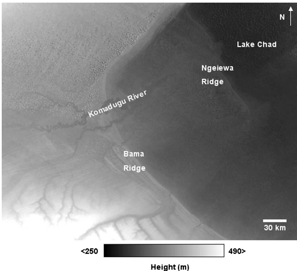
Figure 7 The Bama Ridge on the southwest shoreline of Lake Chad. A well-developed beach ridge complex is evident to the south of the Komadougou River known as the Bama Ridge in Nigeria. To the north of the river is a set of well-developed lake terraces. The elevations of all these shoreline landforms are shown in Table 1
