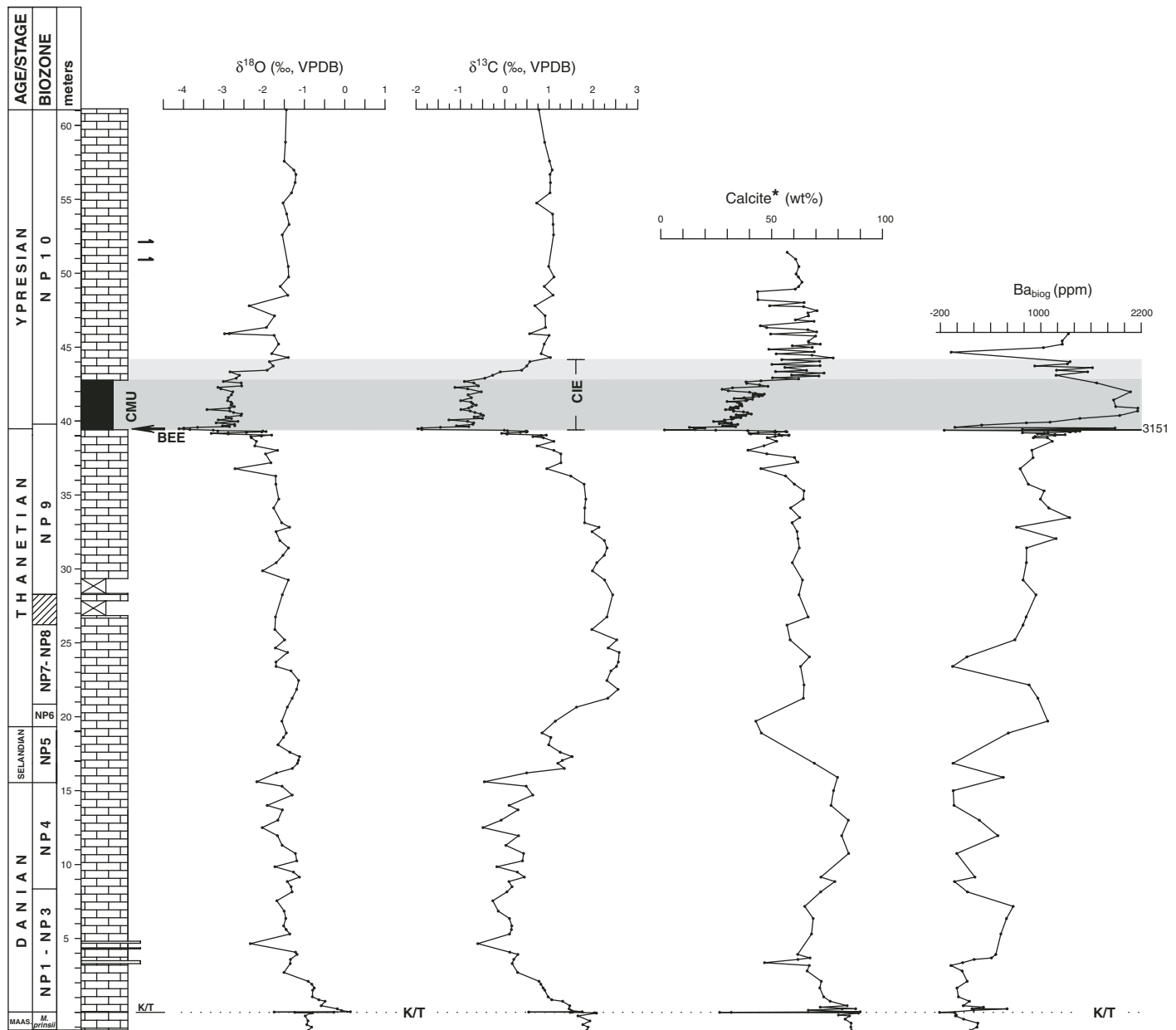
Figure 9. Simplified columnar log, calcareous nannofossil biostratigraphy, stable isotopes stratigraphy ( \delta^{13}\text{C} and \delta^{18}\text{O} measured on bulk sample), \text{CaCO}_3 and \text{Ba}_{\text{biol}} of the entire late Maastrichtian–early Eocene Forada section. For detailed data on \text{Ba}_{\text{biol}} , see Figure 11. Shaded band denotes the interval enclosing the basal Eocene carbon isotope excursion (CIE). Calcite in the interval -122/+3205 cm was determined by recalculating chemical data (CaO and loss on ignition), whereas calcite in the interval +3252/+5142 cm was determined by coulometry. Analytical data are reported in Tables DR1, DR2, and DR3 (see text footnote 1). VPDB—Vienna Pee Dee belemnite standard; BEE—benthic extinction event; CMU—clay marl unit; K/T—Cretaceous-Tertiary boundary.
