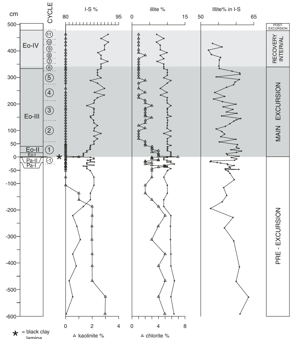
Figure 12. Clay mineral assemblage in the late Paleocene and basal Eocene of the Forada section. The illite component of illite-smectite mixed layer is also reported (illite% in I-S). The clay mineral (<2 \mu m) variations across the Paleocene-Eocene thermal maximum are controlled by the long-term decrease of I-S upward, coupled with decrease of chlorite + illite. Also the content of illite in I-S varies from base to top, but with rather scattered values in the central part of the section. The kaolinite anomaly at the Paleocene-Eocene boundary reported by some authors (see text) is hardly detectable in the Forada section because kaolinite is at trace levels at the base of the section and is undetectable in the upper part.
