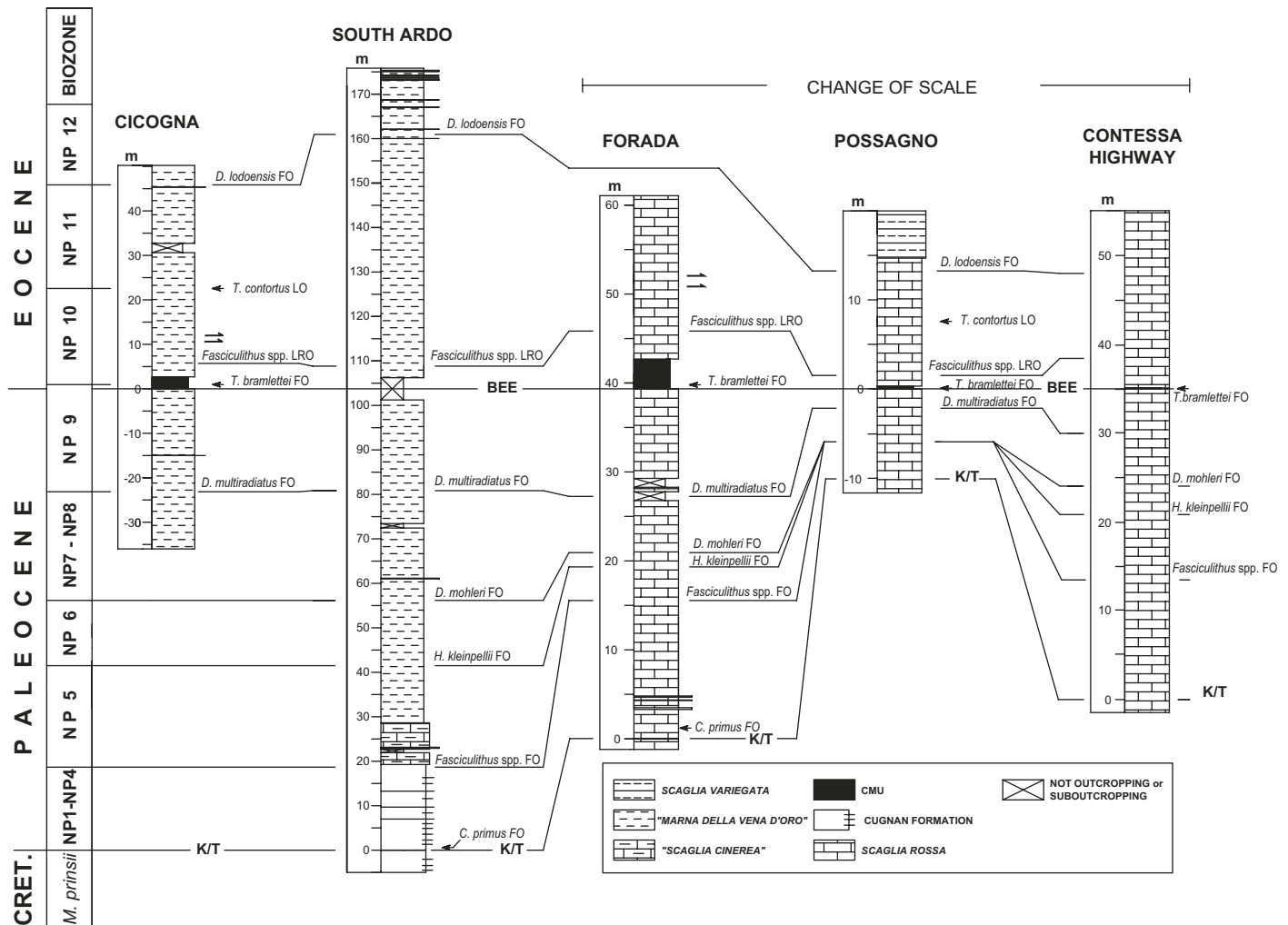
Figure 7. The simplified stratigraphy of the sections studied here (located in Fig. 1) and correlation with the classical sections of Possagno (Veneto region) and the Contessa Highway (Umbria-Marche region, central Italy) based on calcareous nannofossil biostratigraphy. Data on Possagno section are after Agnini et al. (2006) and those on Contessa Highway are after Monechi and Thierstein (1985). Note the change of thickness scale to accommodate the vastly different linear sedimentation rates among sections. FO—first occurrence; LO—last occurrence; LRO—last rare occurrence; BEE—benthic extinction event; CMU—clay marl unit; K/T—Cretaceous-Tertiary boundary; M. — Micula ; D. — Discoaster ; H. — Heliolithus ; C. — Cruciplacolithus ; T. — Tribrachiatulus .
