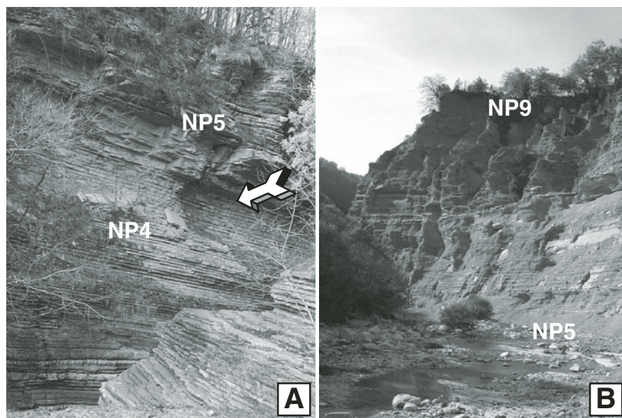
Figure 5. Ardo section. (A) View of the Danian portion of the Cugnan Formation that outcrops close to the Ardo gorge ("Brent Grande"). The arrow indicates the first occurrence (FO) of Fasciculithus spp., which approximates the Danian-Selandian boundary (e.g., Schmitz et al., 1998). Total thickness of outcrop in photograph is ~20 m. (B) View of the Selandian and Thanetian (zone NP5 to zone NP9) in the Ardo section. Total thickness of outcrop in photograph is ~65 m.
