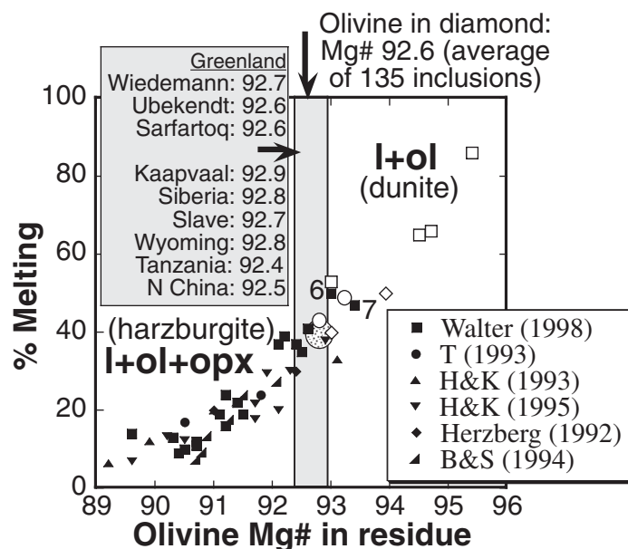
Figure 3. Degree of melting in experiments related to Mg# of residual olivine. Filled symbols refer to residual olivine and orthopyroxene (+ clinopyroxene/garnet at <30\% melting), leaving a harzburgite residue (filled squares marked “6” and “7” are for experiments at 6 and 7 GPa; see text). Open symbols refer to residual olivine only, leaving a dunite residue. Stippled circle is degree of melting as calculated for Wiedemann xenoliths with average olivine Mg# of 92.7 (Bernstein et al., 1998). Bracket at Mg# of 92.4–92.9 is composition of average olivine from cratonic xenolith suites. Data sources for xenoliths and diamond inclusions can be found in the GSA Data Repository (see footnote 1). I—liquid; ol—olivine; opx—orthopyroxene.
