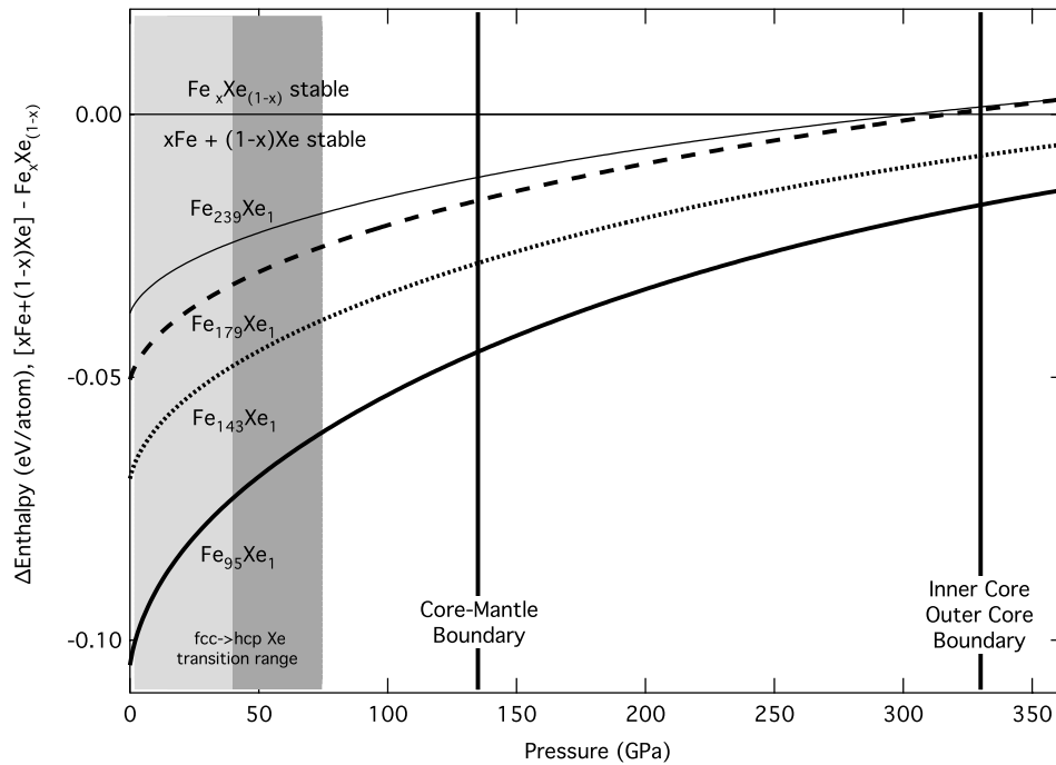
Figure 1. Difference in the enthalpy of the pure elements Fe and Xe compared with the Fe-Xe alloy versus pressure: x\text{Fe} + (1-x)\text{Xe} \rightleftharpoons \text{Fe}_x\text{Xe}_{(1-x)} , where x is a value between 0.9896 and 0.9958 (96- to 240-atom supercells). Curves are labeled for the different Xe concentrations: \text{Fe}_{0.9958}\text{Xe}_{0.0042} ( \text{Fe}_{239}\text{Xe}_1 , ~9700 ppm, thin); \text{Fe}_{0.9944}\text{Xe}_{0.0056} ( \text{Fe}_{179}\text{Xe}_1 , ~13,000 ppm, dashed); \text{Fe}_{0.9931}\text{Xe}_{0.0069} ( \text{Fe}_{143}\text{Xe}_1 , ~16,000 ppm, dotted); and \text{Fe}_{0.9896}\text{Xe}_{0.0104} ( \text{Fe}_{95}\text{Xe}_1 , ~24,000 ppm, thick). For positive values the \text{Fe}_x\text{Xe}_{(1-x)} alloy is energetically favored over the pure elements. The shaded areas represent the fcc-to-hcp phase transition pressure regime: light (1.5–40 GPa [Errandonea et al. , 2002]) and dark (14–75 GPa [Jephcoat et al. , 1987]). The seismically derived core-mantle and inner core–outer core boundary pressures are shown for reference [Dziewonski and Anderson, 1981].
