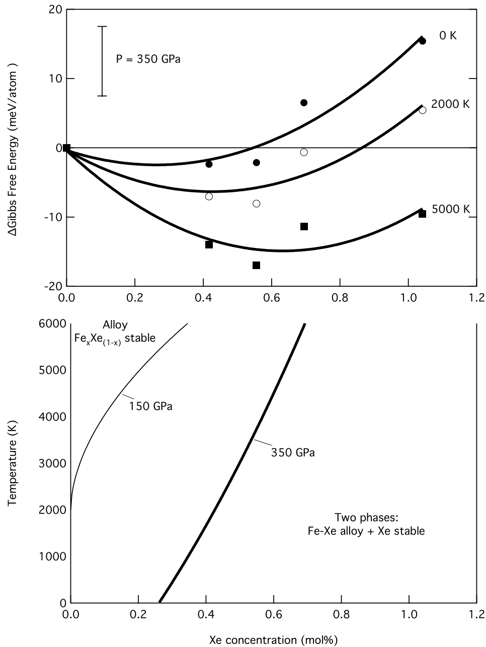
Figure 2. (top) Difference in the Gibbs free energy of the pure elements Fe and Xe compared to the Fe-Xe alloy versus Xe concentration (mol %) at 350 GPa: x\text{Fe} + (1-x)\text{Xe} \rightleftharpoons \text{Fe}_x\text{Xe}_{(1-x)} , where x is a value between 0.9896 and 1.000 at 0 K (solid circles), 2000 K (open circles), and 5000 K (squares). Labeled curves through the data are third-order polynomial fits. The minima of each polynomial fit are used to construct the phase diagram below. A representative error bar is shown for energy convergence uncertainty ( \pm \sim 5 meV). (bottom) Fe-Xe alloy phase diagram of temperature versus Xe concentration. Thick curve delineates the stability boundary between the Fe-Xe alloy and a two-phase space at 350 GPa. For comparison we also include the boundary at 150 GPa (thin curve). To the left of each curve the Fe-Xe alloy is stable, whereas to the right of each curve a mixed region of Fe-Xe alloy and Xe phases are stable. The curvature of the phase boundaries is determined by the quality of the polynomial fit from above.
