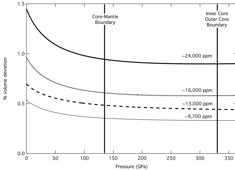
Figure 3. Percent volume difference, 100[V(\text{Fe}_x\text{Xe}_{1-x}) - V(\text{Fe})]/V(\text{Fe}) , versus pressure for the 96-, 144-, 180-, and 240-atom supercells. Curves are labeled according to Xe concentrations: see Figure 1. The seismically derived core-mantle and inner core-outer core boundary pressures are shown for reference [Dziewonski and Anderson, 1981].
