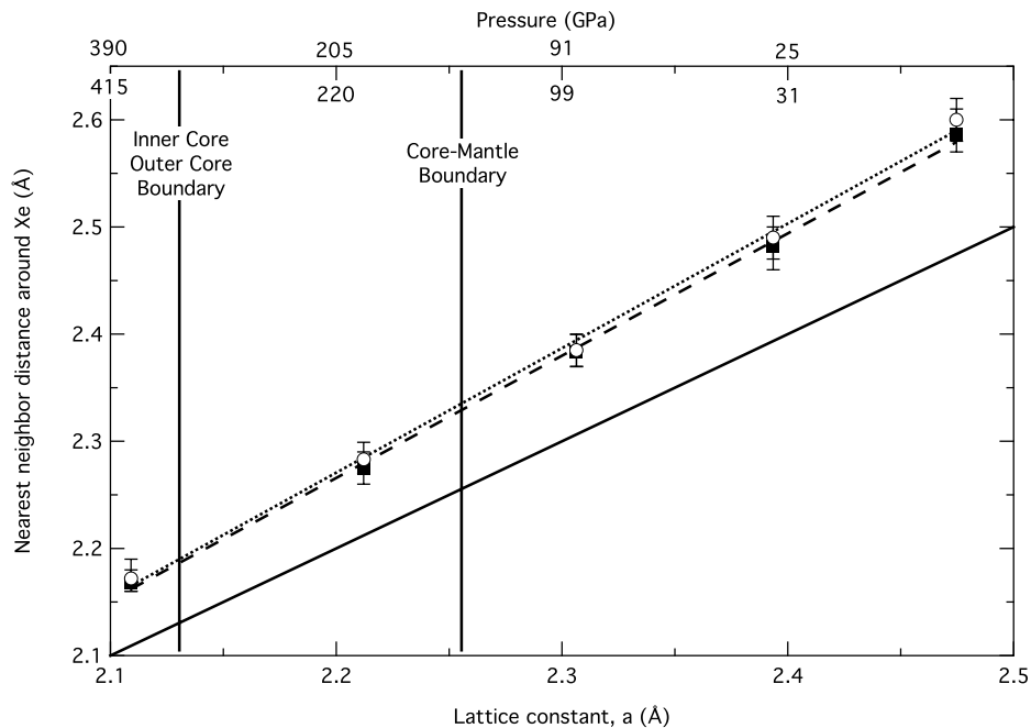
Figure 4. Nearest-neighbor distance around Xe versus lattice constant for the 48-atom (squares) and 180-atom (circles) supercells: \text{Fe}_{0.9792}\text{Xe}_{0.0208} and \text{Fe}_{0.9944}\text{Xe}_{0.0056} . Error bars give the spread around the average nearest-neighbor value. The dotted (dashed) lines yield a best fit line to the 180-atom (48-atom) supercells; the solid line is the 1:1 relation between nearest-neighbor distance and lattice constant. Corresponding pressures are given for the Fe-Xe supercells along the top (180-atom) and bottom (48-atom) of the top axis. With increasing pressure the nearest-neighbor distance gets smaller and more like the lattice constant. The seismically derived core-mantle and inner core-outer core boundary pressures are shown for reference [Dziewonski and Anderson, 1981].
