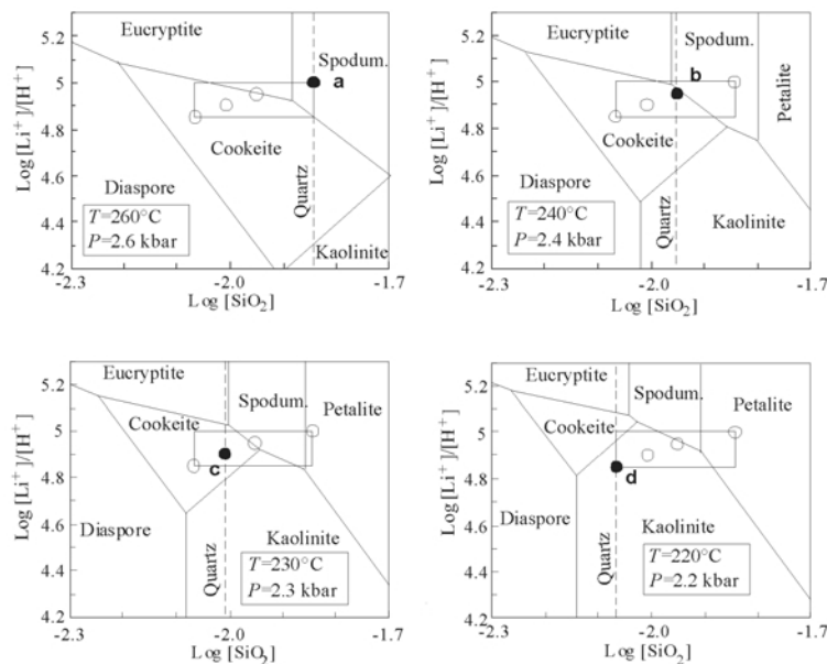
Figure 12. The diagram of \log(a_{Li^+}) + \text{pH} vs. \log(a_{\text{SiO}_2}) as a representation of the stability of cookeite.
