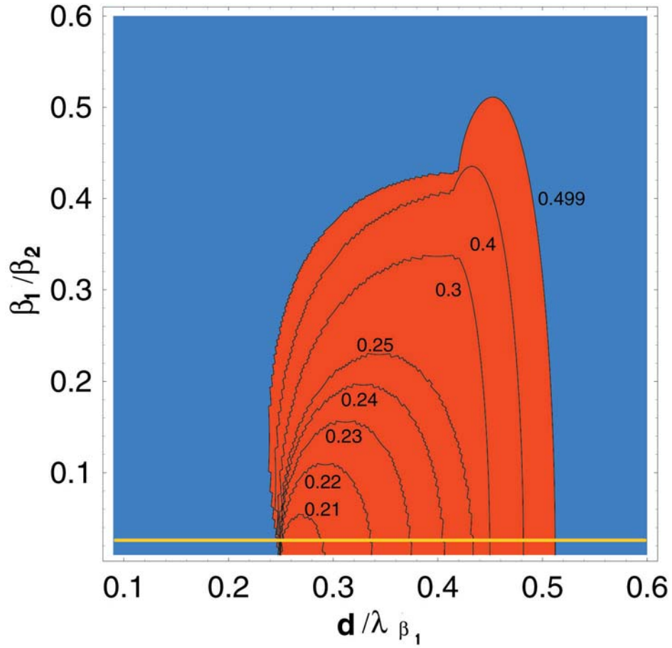
Fig. 3. 2D graph of the range of prograde motion (red) as a function of d/\lambda_{\beta_1} and \beta_1/\beta_2 for different values of v_1 (contours). Note that \beta_1 = 0.0592 km/s and v_2 = 0.2498 are held constant.
