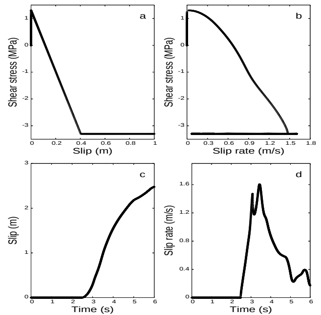
Figure 7. Numerical solutions at a fault point located at 6 km from the end of the nucleation zone.
