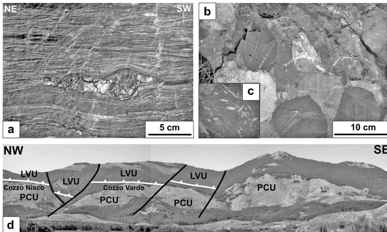
Fig. 5. (a) Intensely deformed calcareous conglomerate of the Pollino–Ciagola Unit in the Campotenese area. (b) Undeformed calcareous conglomerate of the Pollino–Ciagola Unit in the Campotenese area. (c) Well-preserved macroforaminifers (nummulites) in calcareous conglomerate of the Pollino–Ciagola Unit (Campotenese area). (d) Tectonic superimposition of the Lungro–Verbicaro Unit onto the Pollino–Ciagola Unit north of Campotenese. The original low-angle contact (white) is offset by late faults (black lines).
