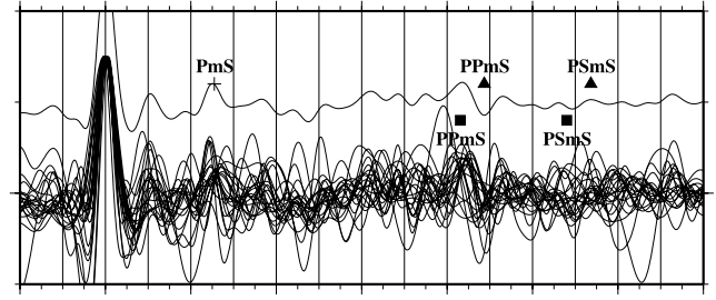
Figure 4. Example receiver functions from three stations. For each station, the single trace at the top of the individual receiver functions is the result of simple time domain summation (without moveout correction) of the individual traces. Triangles are theoretical arrival times for PP\dot{m}S and PS\dot{m}S calculated using equations (2) and (3) by taking p = 5.0 s/deg, V_p = 6.5 km/s, and \phi = 1.73 . H in the equations is calculated based on the observed arrival times of P\dot{m}S . Squares are theoretical arrival times calculated using \phi = 1.80 . The rightward shift of the observed reverberations relative to the triangles for sa24 and sa37 suggests that the actual \phi is smaller than 1.73. For sa59, the similarity between the observed and predicted arrival times for \phi = 1.80 (squares) suggests that the actual \phi is close to 1.80.
