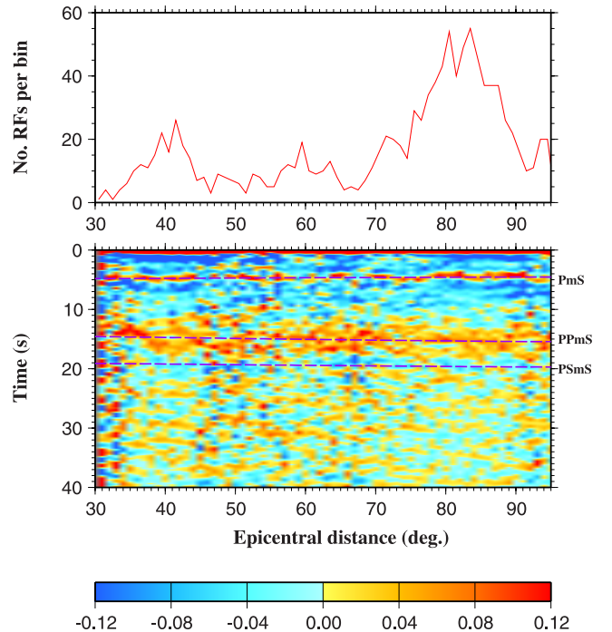
Figure 3. (bottom) Binned and stacked 1544 radial receiver functions used in the study. Dashed lines are predicted moveout curves for PmS , PPmS , and PSmS calculated on the basis of the IASP91 Earth model [Kennett and Engdahl, 1991] with a Moho at 35 km depth. Amplitudes are normalized to P wave amplitudes on radial receiver functions. (top) Number of receiver functions per bin.
