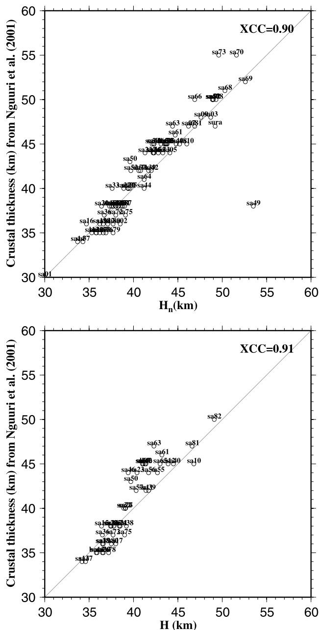
Figure 12. Comparison of crustal thickness measurements obtained by this study and those by Nguiri et al. [2001]. (top) Crustal thicknesses obtained using a fixed \phi = 1.73 , and (bottom) crustal thicknesses obtained by searching for the optimal pair of (H, \phi) .
