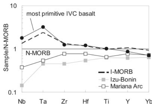
Fig. 12. Comparison of HFSE, Y and Yb abundances in the most primitive IVC basalt with N-MORB (Sun & McDonough, 1989), I-MORB (Price et al. , 1986; Rehkaemper & Hofmann, 1997; Chauvel & Blichert-Toft, 2001) and other island arc lavas: Izu–Bonin (Taylor & Nesbitt, 1998) and Marianas arc (Elliott et al. , 1997).
