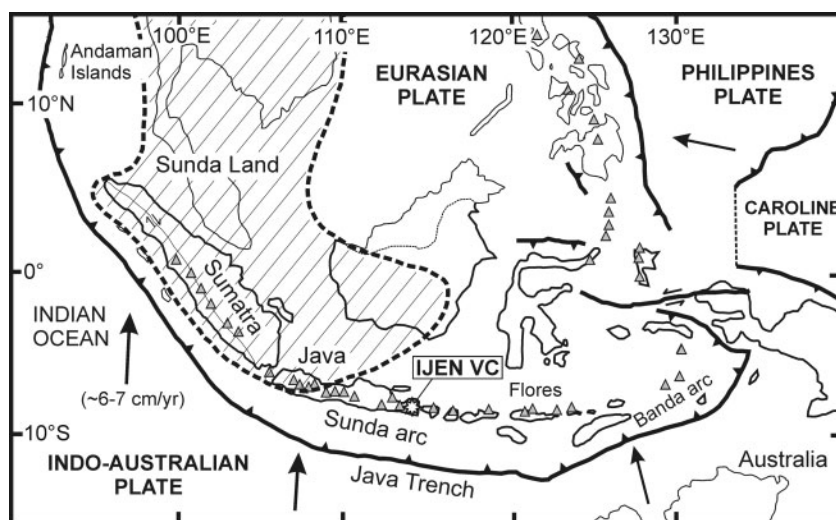
Fig. 1. Tectonic setting of Indonesia [modified from Hoffmann-Rothe et al. (2001)], showing the location of Ijen Volcanic Complex (open star). Black arrows represent the directions of plate movement. Convergence rate of the Indo-Australian Plate and Eurasian Plate from Chase (1978), DeMets et al. (1990) and Tregoning et al. (1994). Grey triangles indicate active volcanoes. Dashed outline of 'Sunda Land' indicates possible extent of continental lithospheric basement (Hamilton, 1979).
