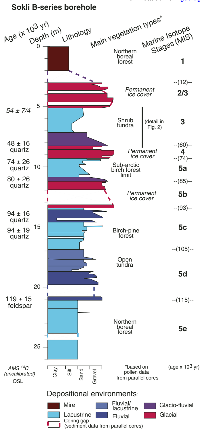
Figure 1. Simplified lithology of Sokli B-series borehole plotted against depth. Changes in depositional environments and main regional vegetation types are shown back to the last interglacial. The independent accelerator mass spectrometry (AMS) 14 C/optically stimulated luminescence (OSL) chronology for the Sokli B-series borehole is indicated on the left, and correlations with the deep-sea record (Martinson et al., 1987) are on the right.
