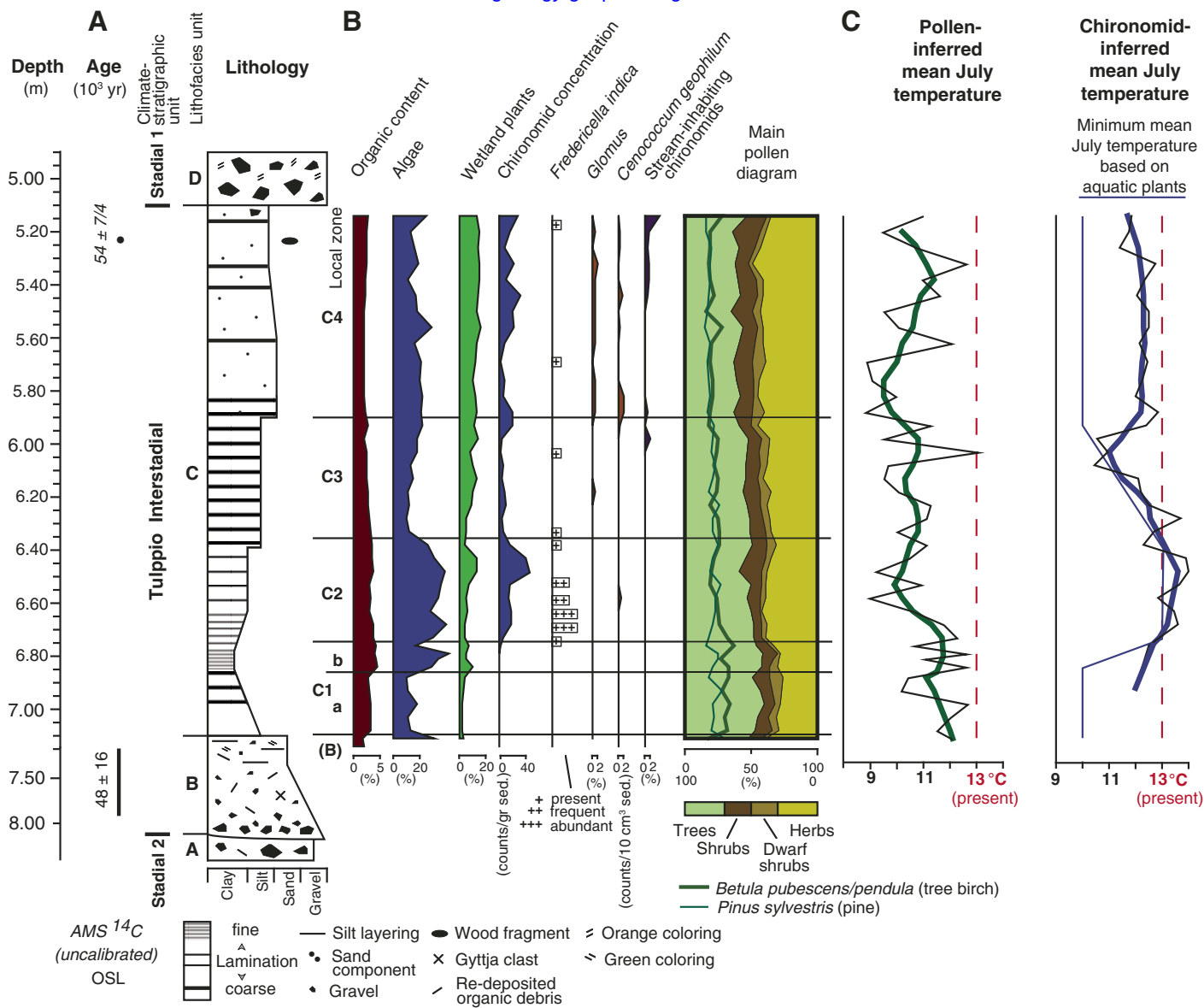
Figure 2. Multiproxy records from Sokli lacustrine sediments of the early part of marine isotope stage (MIS) 3 ca. 50 ka. A: Lithological column for depth interval 4.90–8.40 m in borehole Sokli B-series and absolute age determinations. Lithofacies units A and D represent glacial till, unit B comprises proglacial gravels and sands fining upward into sands interlayered with silts, and C is laminated lacustrine silts and clays. The accelerator mass spectrometer (AMS) ^{14}\text{C} dating (U/C 14712) was carried out on terrestrial plant macrofossils. OSL—optically stimulated luminescence. B: Selected proxy indicators from multiproxy analysis that reflect local environmental changes and changes in regional vegetation during local zones C1–C4. C: Curves of pollen- and chironomid- (aquatic insect) inferred mean July air temperatures, with Loess (locally weighted regression) smoother (span = 0.2) superimposed on inferred values to highlight major trends. Chironomid-based temperature curve additionally shows minimum mean July temperature values inferred from specific aquatic plant taxa (thin blue line). Present \sim 13^\circ\text{C} mean July temperature at Sokli is indicated for reference.
