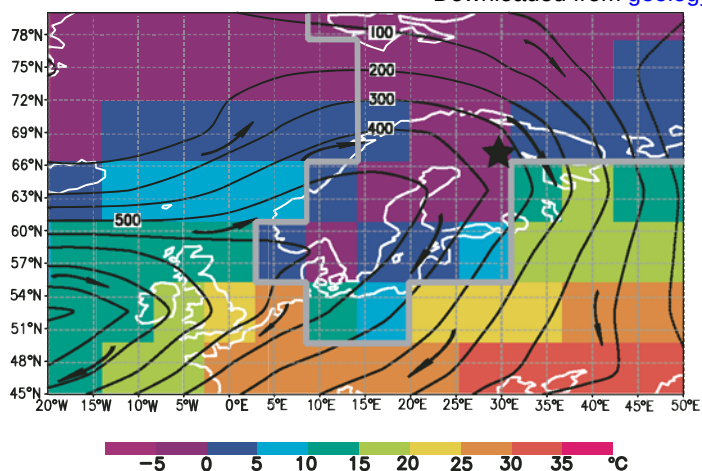
Figure 3. Simulated mean July surface air temperature over northern and middle parts of Europe. Contour lines represent geopotential height at 800 hPa, while arrows give schematic view of wind direction in lower atmosphere. Extent of the prescribed marine isotope stage 3 Scandinavian Ice Sheet is indicated in gray; star shows location of Sokli. Note that the model is not suitable for analyzing results at the grid-cell scale because of its low spatial resolution: the model is designed for continental and subcontinental scales.
