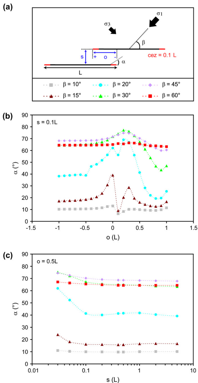
Fig. 11. (a) Fault configuration and symbols corresponding to various \beta values; Plots showing the relationships between (b) the kink angle \alpha and the fault overlap “ o ” and (c) \alpha and the fault separation “ s ”.
