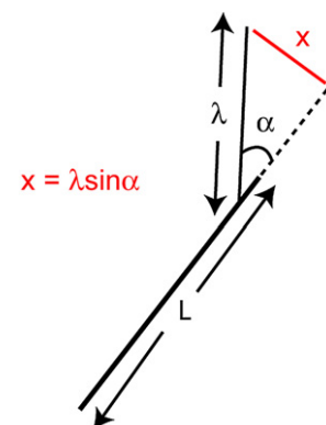
Fig. 12. Relationships between the splay length \lambda , the kink angle \alpha and the distance “ x ” perpendicular to the fault to which the splays propagates.
