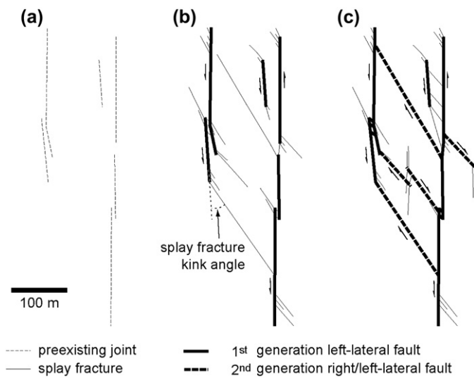
Fig. 2. Conceptual model for the evolution of the strike-slip fault networks in the Valley of Fire State Park, Nevada. (a) Pre-existing joints prior to, or at the earliest phase of, faulting. (b, c) Progressive stages of splay fracturing and sequential shearing of splay fractures that evolve into two sets of left- and right-lateral strike-slip faults in an apparent conjugate pattern. Simplified from Flodin and Aydin (2004a).
