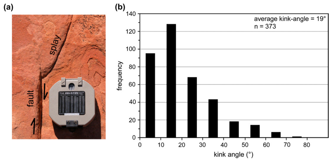
Fig. 6. (a) Photograph of an isolated fault configuration. (b) Corresponding kink angle distribution.
