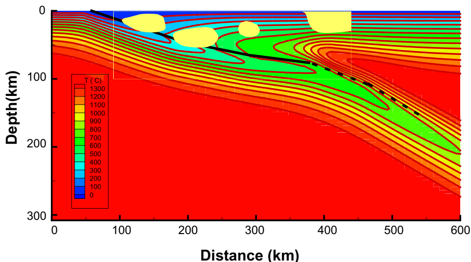
Figure 10. Thermal structure of subducting Cocos plate along profile A-A' after Rüpkke et al. [2004]. Conductive zones are added from Figure 6.
