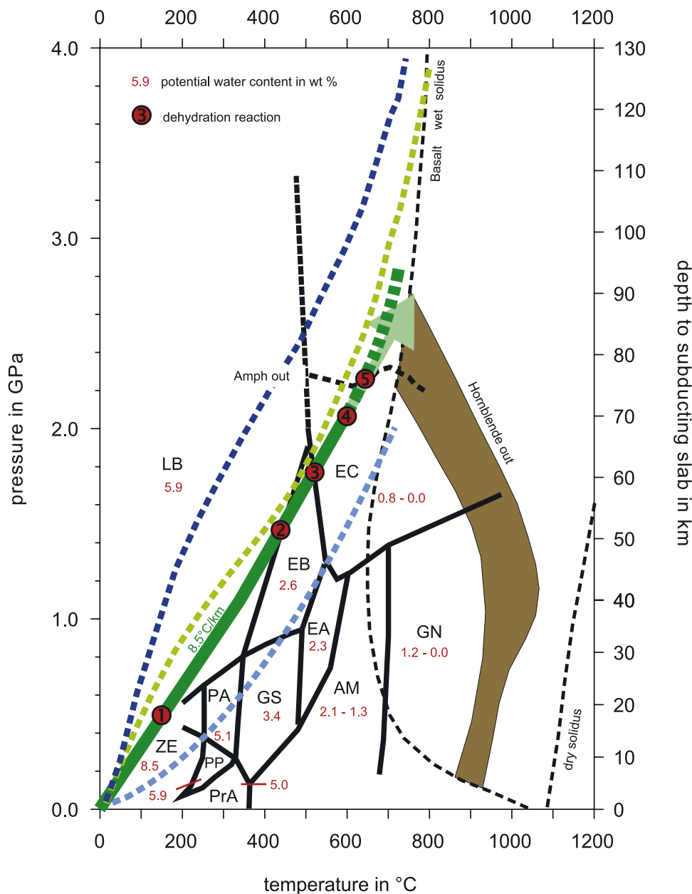
Figure 9. P,T conditions at the top of the subducting Cocos plate as proposed from the assumed relation between facies transitions and observed conductivity anomalies (dark green line). In comparison, geotherms are shown as adopted for the Cocos plate from thermal models by Peacock [1996] (modified from p-T path 2 in his Figure 4B, dashed light blue line) and from the thermal model shown in Figure 10 after Rüpke et al. [2002] (dashed bright green line). The dashed dark blue line results from the same model but excludes the effect of moderate shear heating (see text). The pressure-temperature diagram of metamorphic facies for a fully hydrated basaltic bulk composition is compiled from Peacock [1993], Peacock et al. [1994], and Schmidt and Poli [1998]. Metamorphic facies abbreviations are AM, amphibolite; EA, epidote-amphibolite; EB, epidote-blueschist; EC, eclogite; GN, granulite; GS, greenschist; LB, lawsonite-blueschist; PP, pumpellyite-actinolite; PrA, prehnite-actinolite; PA, pumpellyite-actinolite; ZE, zeolite facies. Note that the segmented depth scale is linearly converted from pressure due to crustal density 2.8 \text{ g cm}^{-3} for 0–40 km depth after Ramirez-Ruiz [1994] and to mantle density 3.3 \text{ g cm}^{-3} for depths >40 km, assuming a constant thermal gradient 8.5^\circ\text{C km}^{-1} of the Cocos plate.
