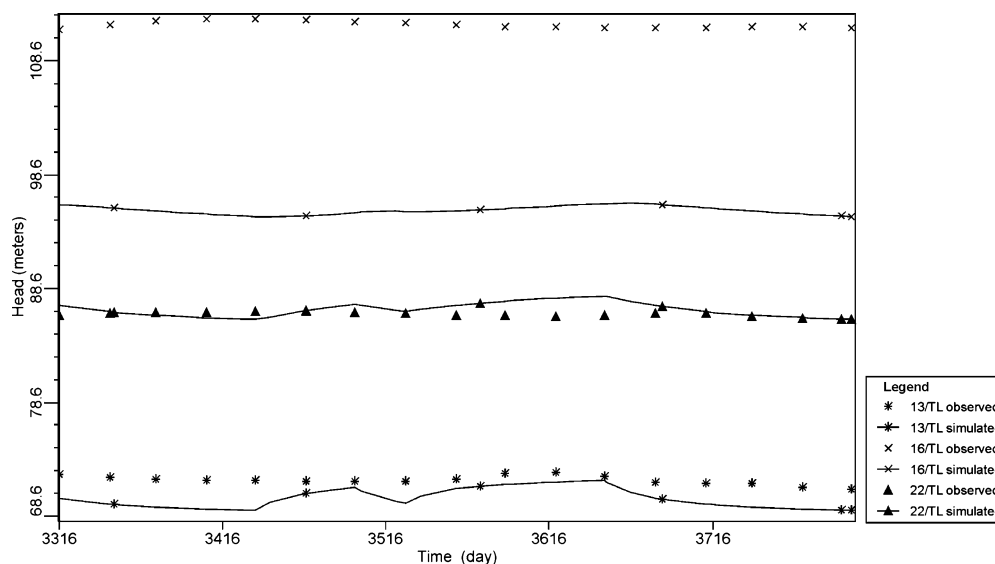
Fig. 8 Hydraulic head fluctuations for upland wells (1970–1971 model). Results are shown for the tenth cycle
