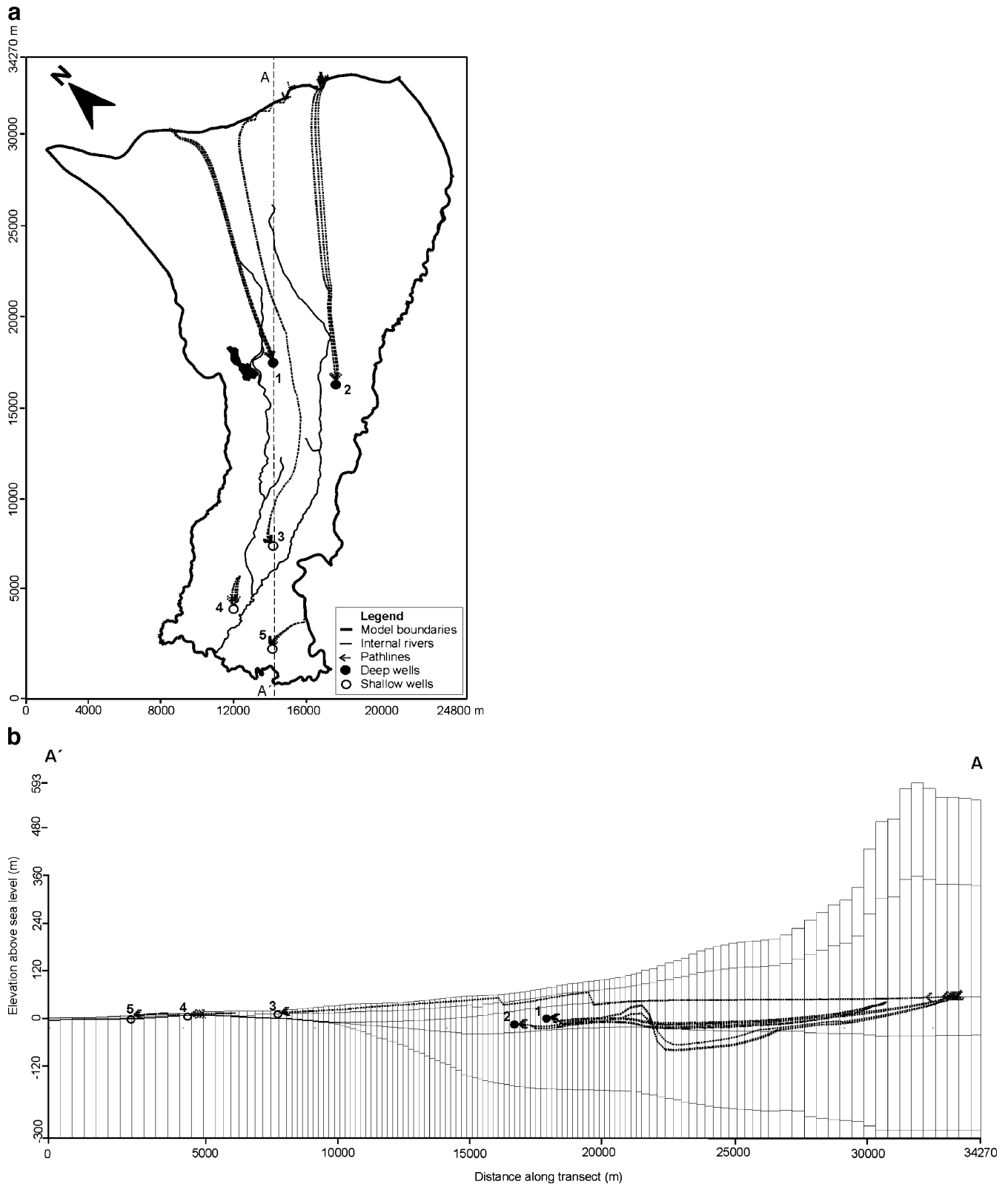
Fig. 11 Particle tracking results: a plan view and b cross section
