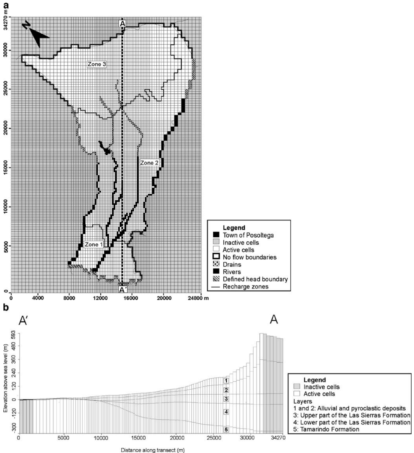
Fig. 3 a Model grid, model boundaries and recharge zones (layer 1). Map in model coordinates (meters). b Model cross section A'A with five grid layers. The top two layers represent the pyroclastic and alluvial deposits, followed by the upper and lower Las Sierras Formation and the Tamarindo Formation, respectively. Map in model coordinates
