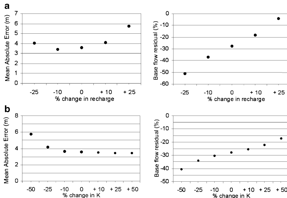
Fig. 9 a Sensitivity analysis for recharge. b Sensitivity analysis for conductivity K of layer 1
