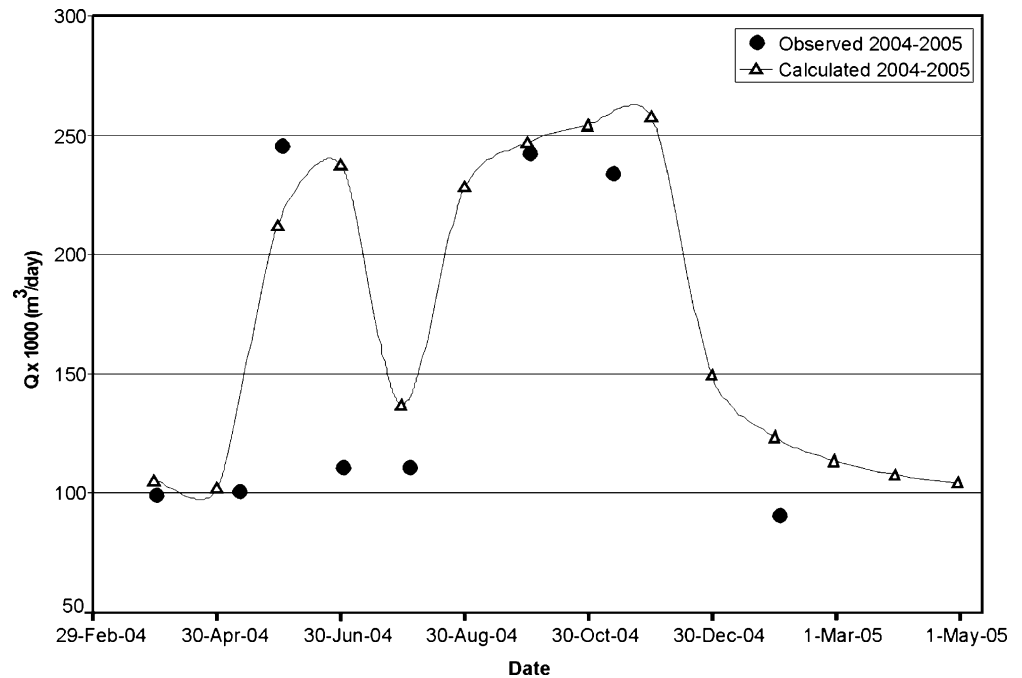
Fig. 6 River base flow ( Q ) calibration for 2004–2005 model
