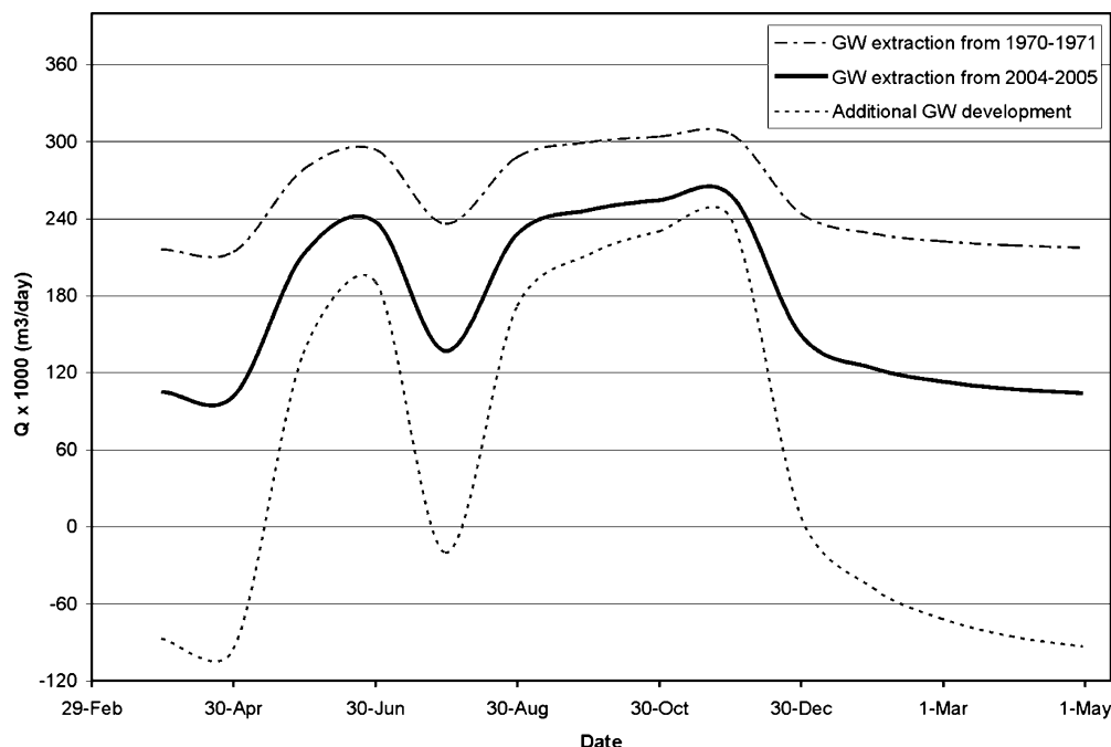
Fig. 10 River base flow ( Q ) simulations for 1970–1971, 2004–2005 and 100% increase in groundwater (GW) extraction. Negative figures indicate a total absence of base flow
