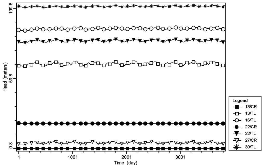
Fig. 7 Hydraulic head values starting from steady-state initial conditions and repeating the 1970–1971 model year recharge and pumping stresses for 10 years. The influence of the initial conditions is not evident after the first simulated year
