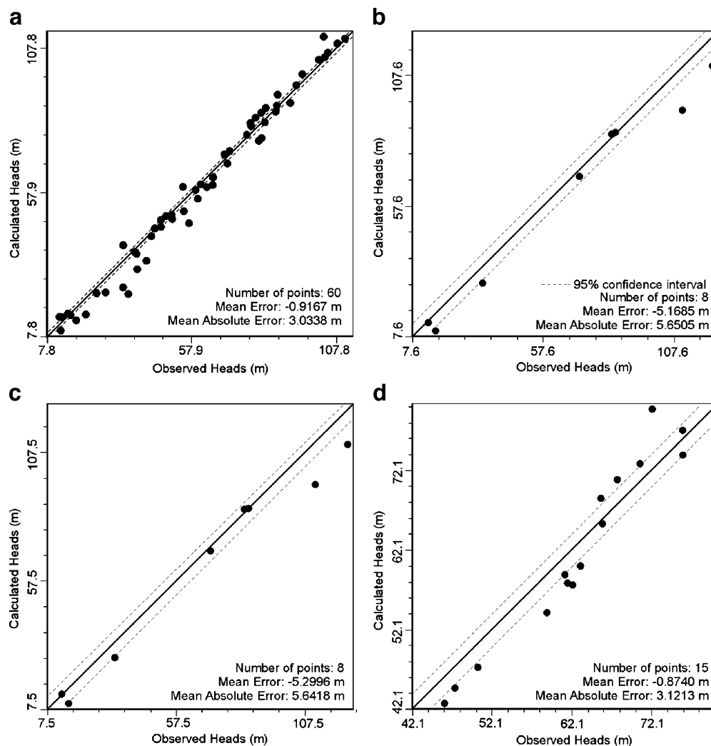
Fig. 4 a Calculated vs. observed hydraulic heads for 1999 model (steady state). For observation well locations, see Fig. 5a. b Calculated vs. observed hydraulic heads for 1965–1975 model (steady state). For observation well locations, see Fig. 5b. c Calculated vs. observed hydraulic heads for the end of the 1971 dry season (April). For observation well locations, see Fig. 5b. d Calculated vs. observed hydraulic heads for the end of the 2005 dry season (April). For observation well locations, see Fig. 5c
