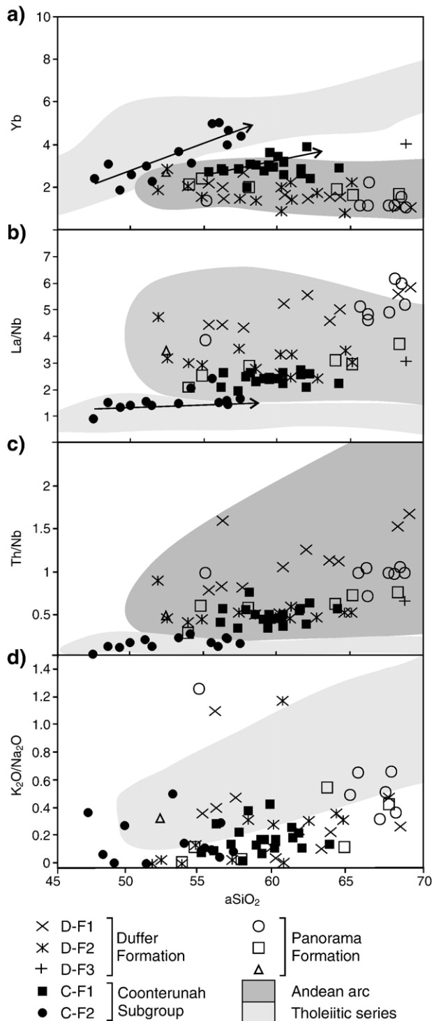
Fig. 5. Variation diagrams showing Yb (ppm), La/Nb, Th/Nb, and \text{K}_2\text{O}/\text{Na}_2\text{O} vs. \text{SiO}_2 (anhydrous) [ a\text{SiO}_2 ] for trace element enriched basalt–dacite units of the Warrawoona Group (Pilbara Supergroup). Shaded field are for a range of subduction related rocks from the Andean arc and for tholeiitic basalts to rhyolites from Iceland (data from the GEOROC database— http://georoc.mpch-mainz.gwdg.de/ ).
