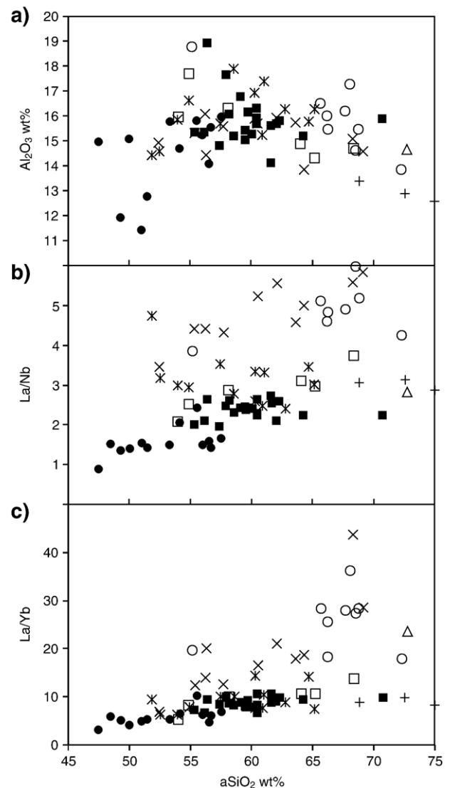
Fig. 6. Variation diagram showing \text{Al}_2\text{O}_3 , La/Nb and La/Yb vs. \text{SiO}_2 (anhydrous) for trace element enriched basalt–dacite units of the Warrawoona Group (Pilbara Supergroup) (symbols as for Fig. 5). With decreasing age (Coonterunah→Duffer→Panorama), the rock groups become generally more silicic and have higher average La/Nb and La/Yb as a result of the presence of increasingly TTG-like rocks.
