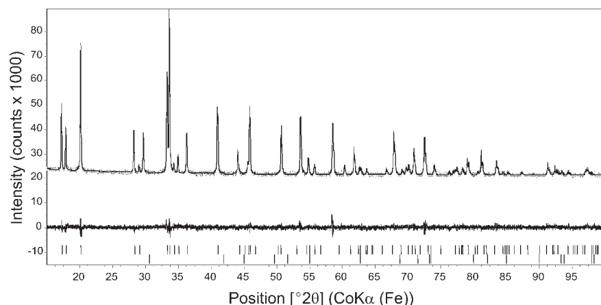
FIGURE 2. Rietveld refinement plot of sample D, (K_{0.350}H_{3.0}O_{0.650})Fe_{2.93}(SO_4)_2(OH)_6 . The sample was refined with two phases (jarosite + alumina). The gray line is the observed data and the solid line is the calculated pattern. The vertical bars mark all possible Bragg reflections ( CoK\alpha_1 and K\alpha_2 ), where upper and lower bar marks are jarosite and alumina, respectively. The difference between the observed and calculated patterns is shown at the bottom.
