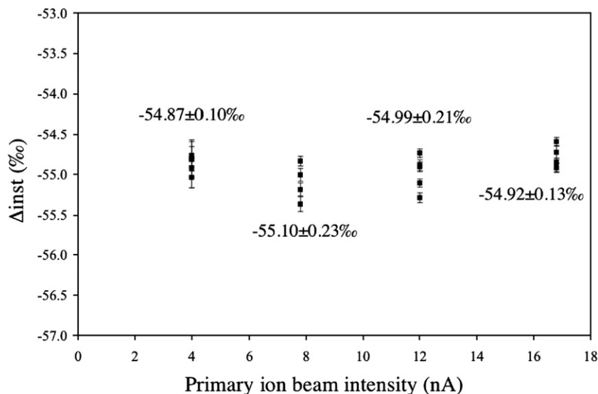
Fig. 4. \Delta_{\text{inst}} values as a function of primary ion beam intensity for BRET 105E reference material measurements. \Delta_{\text{inst}} was calculated using an arbitrary ^{44}\text{Ca}/^{40}\text{Ca} of 0.212116 (no absolute ratio is certified yet for carbonate reference material). We obtained average 2\sigma_n values of \pm 0.2\% indicating that \Delta_{\text{inst}} values can be considered as constant over a primary beam intensity ranging from 4 to 16.8 nA.
