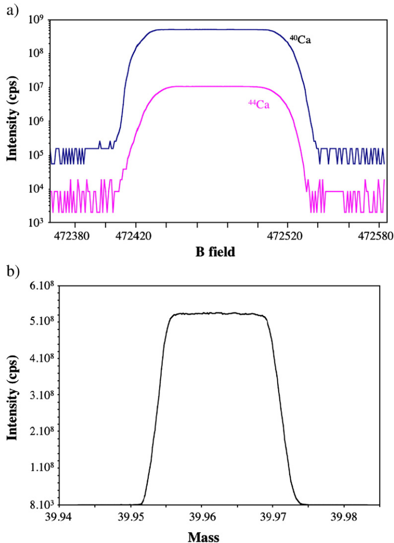
Fig. 1. High resolution mass spectra showing in a) the ^{40}\text{Ca}^+ and ^{44}\text{Ca}^+ peaks in multicollection and on a log scale, and in b) at mass 40, the ^{40}\text{Ca}^+ peak on a linear scale.
