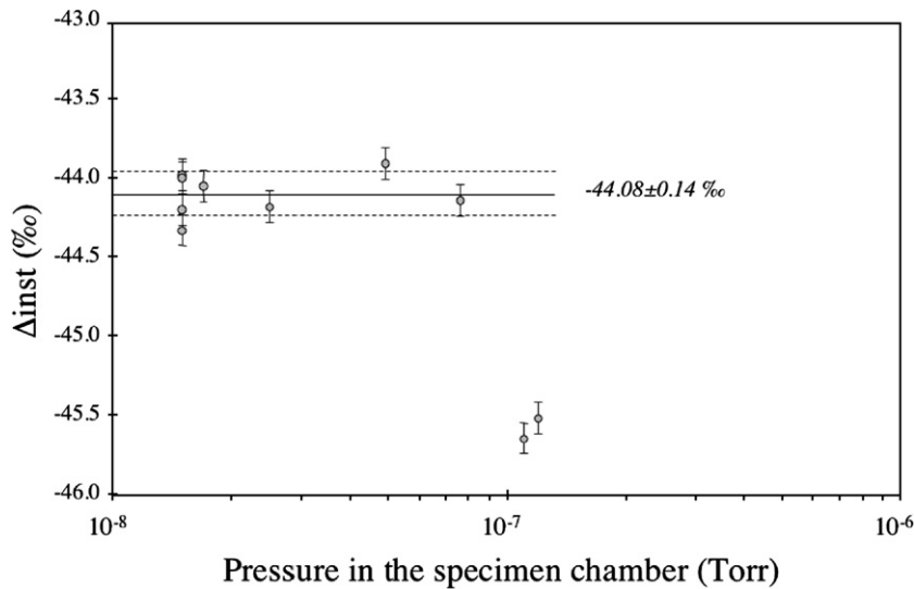
Fig. 3. \Delta_{\text{inst}} measured on the MEX standard during the drop of the pressure in the specimen chamber immediately following introduction of the sample. The magnitude of \Delta_{\text{inst}} decreases by \approx 2.5\% over the 15-min pumping time. The solid line indicates the mean \Delta_{\text{inst}} ( \bar{\Delta}_{\text{inst}} ) value calculated over measurements performed at pressures below 8 \times 10^{-8} Torr. The dashed lines indicate \bar{\Delta}_{\text{inst}} + 1\sigma and \bar{\Delta}_{\text{inst}} - 1\sigma values, where \sigma is the standard deviation obtained for these measurements. Below a pressure of 8 \times 10^{-8} Torr, \Delta_{\text{inst}} values can be considered constant within a standard deviation of \pm 0.14\% , which does not exceed the 1\sigma external precision of measurements.
