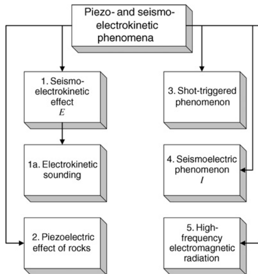
Figure 1. Types of piezoelectric and seismoelectrokinetic phenomena.
