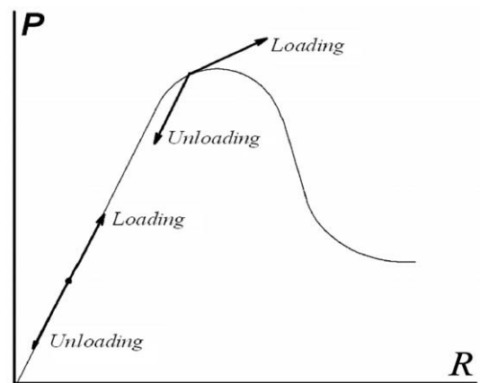
Fig. 1. Schematic view of the constitutive law of a brittle mechanic system. P and R correspond to the load and response of a mechanic system. The response is linear to the load and unload when the load is well below the strength of the system, and becomes nonlinear when the system is close to failure.
