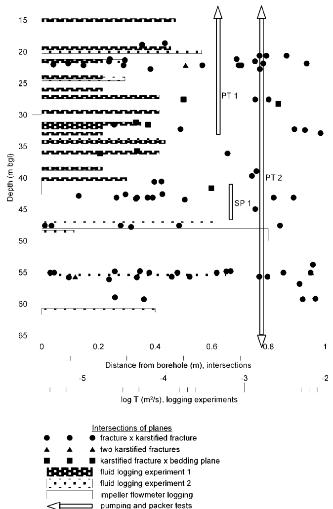
Fig. 17 Results from the fracture analysis in relation to the results from the hydraulic experiments. The main flowing features—high transmissivity ( T )—correlate well with the levels where at least one of the intersecting features is karstified. This correlation diminishes with distance of the intersection to the borehole wall
