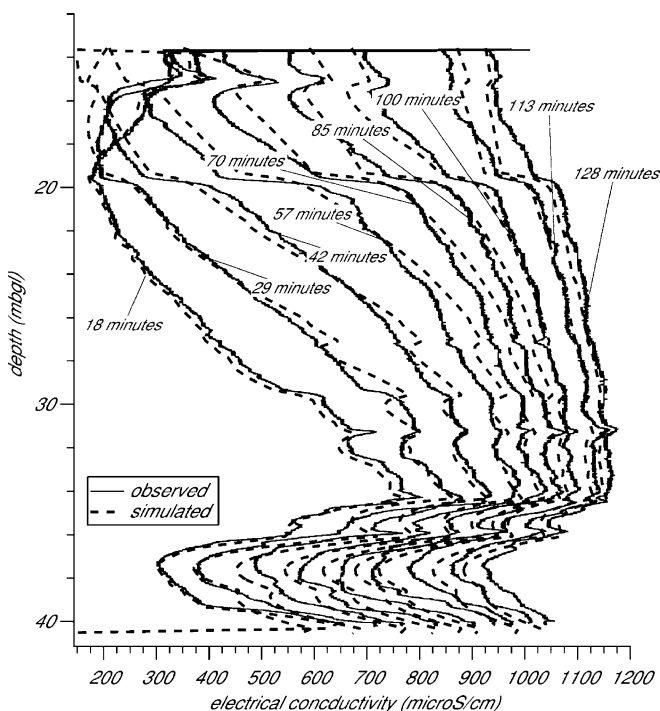
Fig. 9 Fluid-logging fit to experiment 1. It represents the consecutive electrical conductivity profiles after flushing and reaching steady state after 18 min
