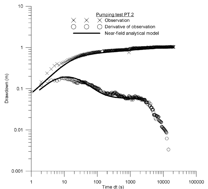
Fig. 7 Log-log plot of drawdown vs. time for pumping test 2
