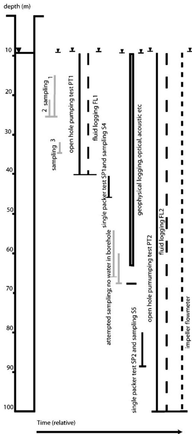
Fig. 6 Borehole with a relative time axis indicating all sampling, logging and testing along with water depth measured at different stages. Markers in grey signify the sampling of the water table on five occasions
