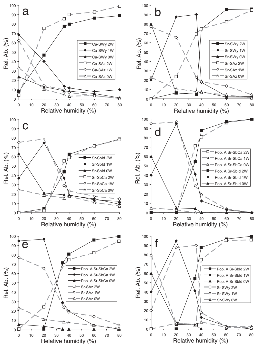
FIGURE 7. Evolution of relative abundance of layer types as a function of RH. (a) Ca-SA z -1 and Ca-SWy-1. (b) Sr-SA z -1 and Sr-SWy-1. (c) Sr-Sbld-1 and Sr-SbCa-1. (d) Population A of Sr-Sbld-1 and Sr-SbCa-1. (e) Sr-SA z -1 and population A of Sr-SbCa-1. (f) Sr-SWy-1 and population A of Sr-Sbld-1. Triangles, diamonds, and squares represent 0W, 1W, and 2W layers. Data for Ca- and Sr-SWy-1 are those reported by Ferrage et al. (2005b). XRD data collection was performed in adsorption conditions at 40, 60, and 80% RH, and in desorption conditions at 0, 20, 35% RH.
