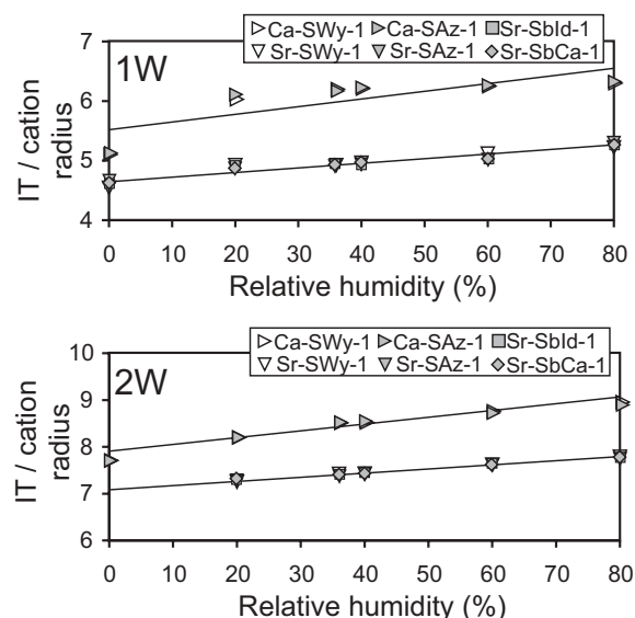
FIGURE 8. Evolution of layer thickness of hydrated layers as a function of RH for all samples including SWy-1 (Ferrage et al. 2005b). Interlayer thickness (IT) is represented by the ratio IT:ionic radius. IT is calculated as the basal distance d_{001} minus the thickness of the 2:1 layer (6.54 Å). Linear regression lines are plotted for each cation and include all samples saturated with this cation.
