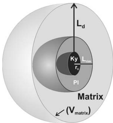
Fig. 7 Schematic figure of different layers forming the local Al-rich domain and its surrounding used for calculation of equilibration volume necessary for the plagioclase rim development
