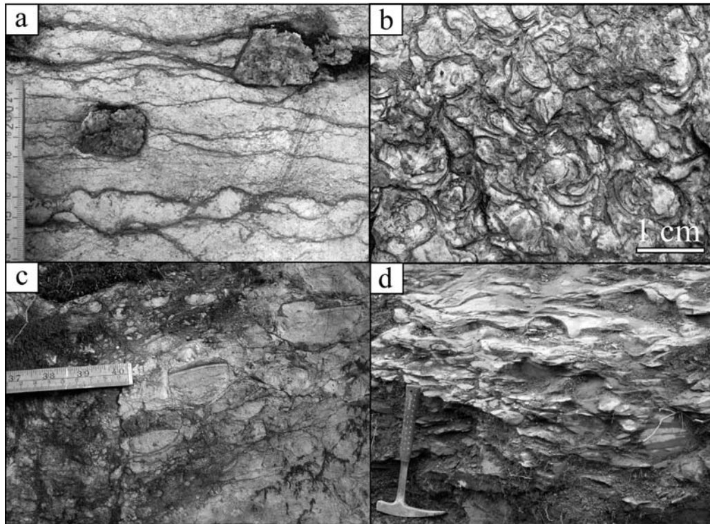
Fig. 4. Outcrops at the Tandsbyn gully, Lockne crater. a) Lithology of the rim facies. A light gray biocalcareneite containing crystalline clasts of the brecciated basement found only on the crater rim. b) Part of the brachiopod coquina bed found in the upper layers in the rim facies. c) The cephalopod facies, a thick-bedded calcilutite with a high abundance of nautiloid conchs. d) The argillaceous facies at the bottom of the Tandsbyn gully characterized by argillaceous limestone nodules set in a hard, slightly fractured mudstone.
