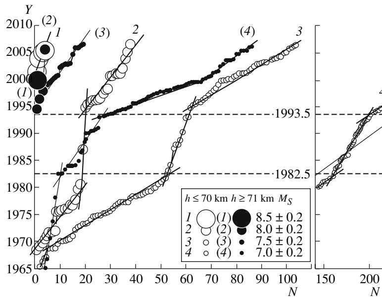
Fig. 2. Cumulative graphs of planetary seismic events with magnitude of 7.0 \pm 0.2 , 7.5 \pm 0.2 , 8.0 \pm 0.2 , and 8.5 \pm 0.2 in the years 1965–2005. (1–4) Linear approximation of the origination of earthquakes with hypocenter not deeper than 70 km; (1)–(4) the same for the seismic events with hypocenter deeper than 70 km.
