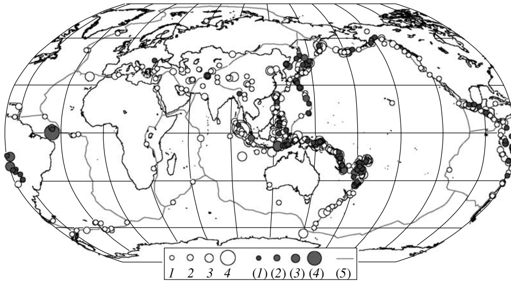
Fig. 1. Epicenters of large earthquakes on the Earth in the years 1965–2005. (1–4) Earthquakes with magnitude of 7.0 \pm 0.2 , 7.5 \pm 0.2 , 8.0 \pm 0.2 , and 8.5 \pm 0.2 and hypocenter h not deeper than 70 km; (1)–(4) earthquakes with the same magnitude and hypocenter h deeper than 70 km; (5) boundaries of lithospheric plates. Only the state boundary of Russia is shown.
