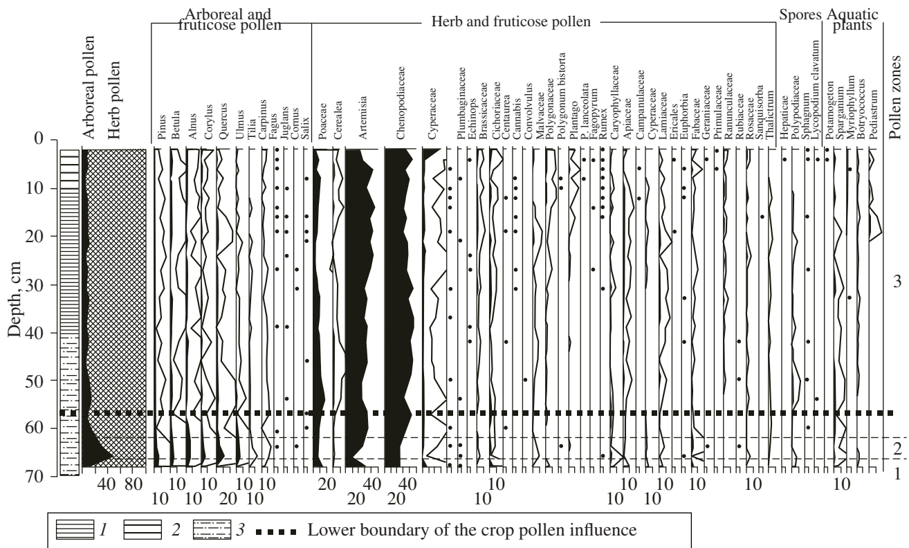
Fig. 3. Spore-and-pollen diagram for the section of bottom sediments from Taganrog Bay, Sea of Azov. Lithology: (1) clayey ooze; (2) silty-clayey and sandy sediment; (3) sand with coquina. Percentages of spectrum components are calculated from the pollen of arboreal and herb species. An additional contour shows the exaggerated content (by 10 times) of minor components.
