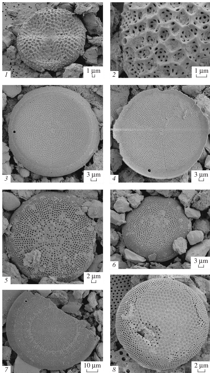
Fig. 2. Dominant diatom species: (1, 2) Actinoptychus senarius (Ehr.) Ehr.; (3–8) a type form and varieties of Actinocyclus octonarius Ehr.
