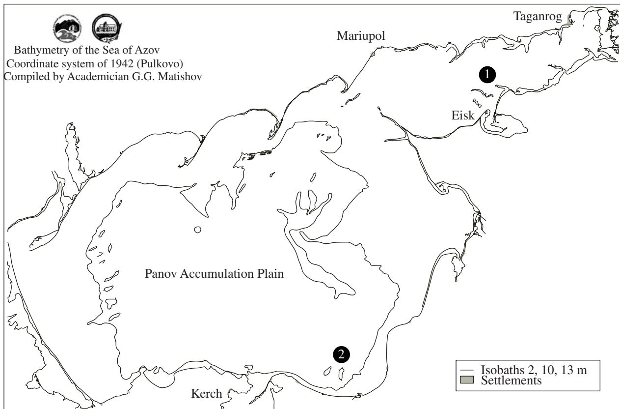
Fig. 1. Bathymetric map of the Sea of Azov with sites of core sampling for (1) palynological and (2) diatom analyses.
