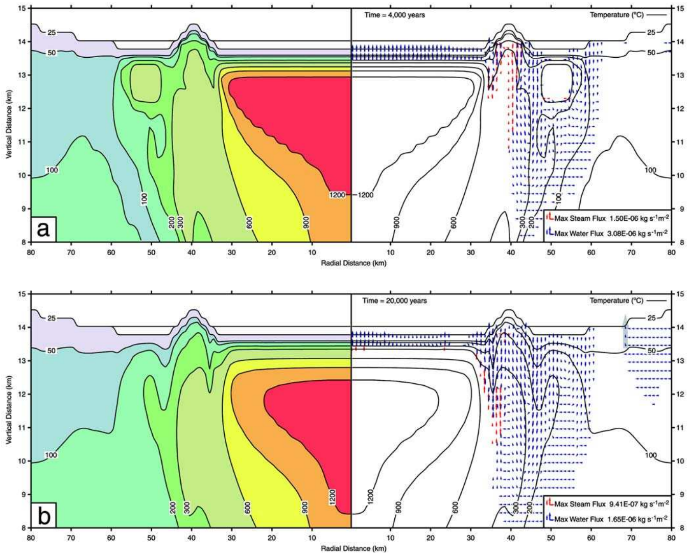
Fig. 3. Results of a numerical simulation of the hydrothermal system at Chicxulub crater. Surface permeability k_0 is 10^{-3} darcies. Black lines are isotherms, labeled in degrees Celsius, and blue and red arrows represent water and steam flux vectors, respectively. The lack of arrows indicates that fluxes are at least 2 orders of magnitude smaller than the maximum flux. The length of the arrows scales logarithmically with the flux magnitude, and the maximum value of the flux changes with each plot. Large gray arrows indicate upward water flow through a fault zone in the crater's modification zone.
