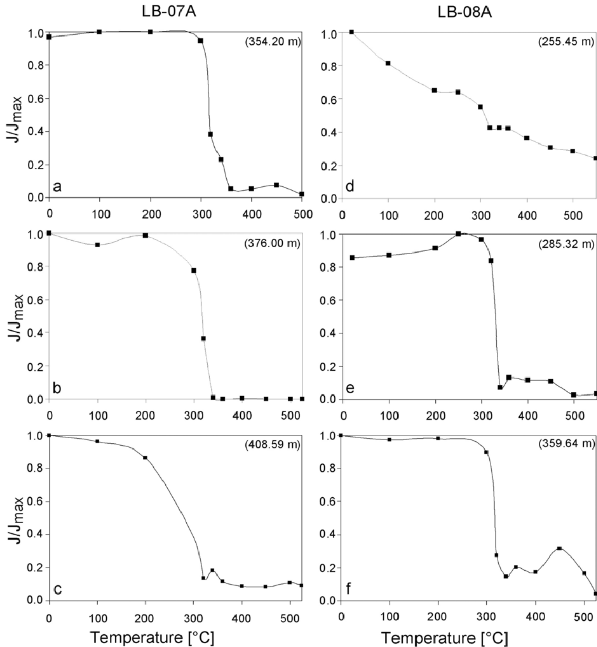
Fig. 4. Intensity decay of the NRM during thermal demagnetization for different depths and lithologies of the LB-07A and LB-08A. a), b), and d) Polymict lithic breccia units. c) Suevite. e) Shale. f) Phyllite.
