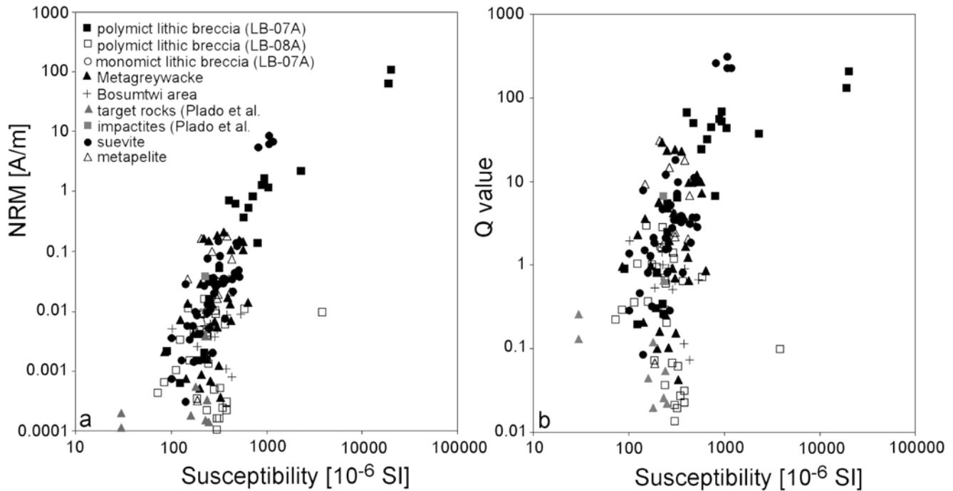
Fig. 7. Natural remanent magnetization (NRM) versus (a) susceptibility and (b) Koenigsberg (Q) ratio versus susceptibility for different impact and target lithologies of the BCDP drill cores and samples from the surface. Bosumtwi area denote different suevites and target lithologies from the surrounding of the crater (kindly provided by A. Deutsch, Münster.)
