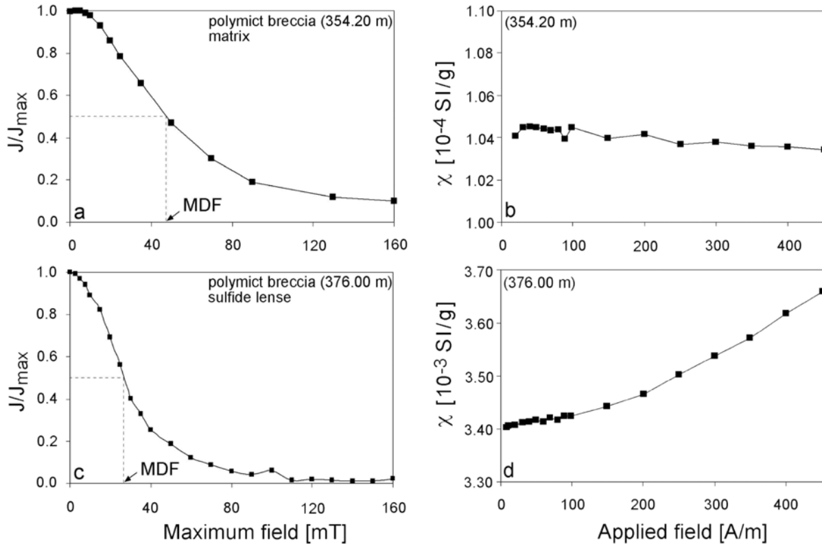
Fig. 5. Alternating field demagnetization of NRM and field-dependence of magnetic susceptibility for the polymict breccia at 354.20 m depth showing high MDF (a) and no field-dependence (b), and for the sulfide lense in the greenschist clast at 376.0 m depth with a lower MDF (c) and a strong field-dependence (d).
