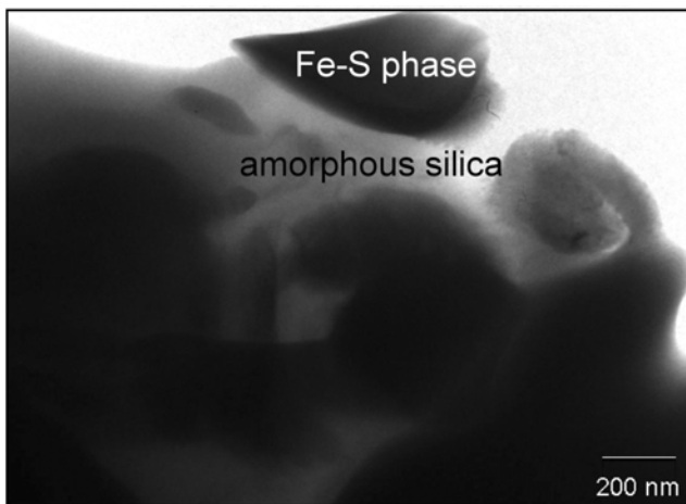
Fig. 8. TEM-bright field image showing Fe sulfide particle (most likely pyrrhotite) in amorphous silica. Polymict lithic breccia from 354.2 m of LB-07A drill core.
