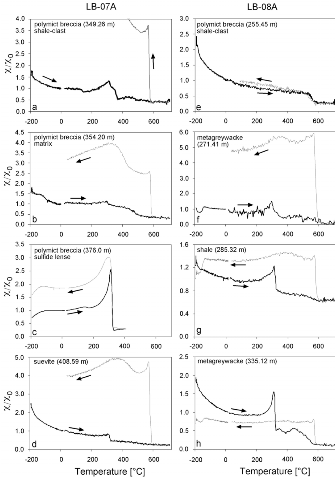
Fig. 3. Normalized susceptibility as function of temperature between -192 and 700 °C. Black line is the heating curve; gray line is the cooling curve (also indicated by arrows). Curie temperatures are summarized in Table 1.
