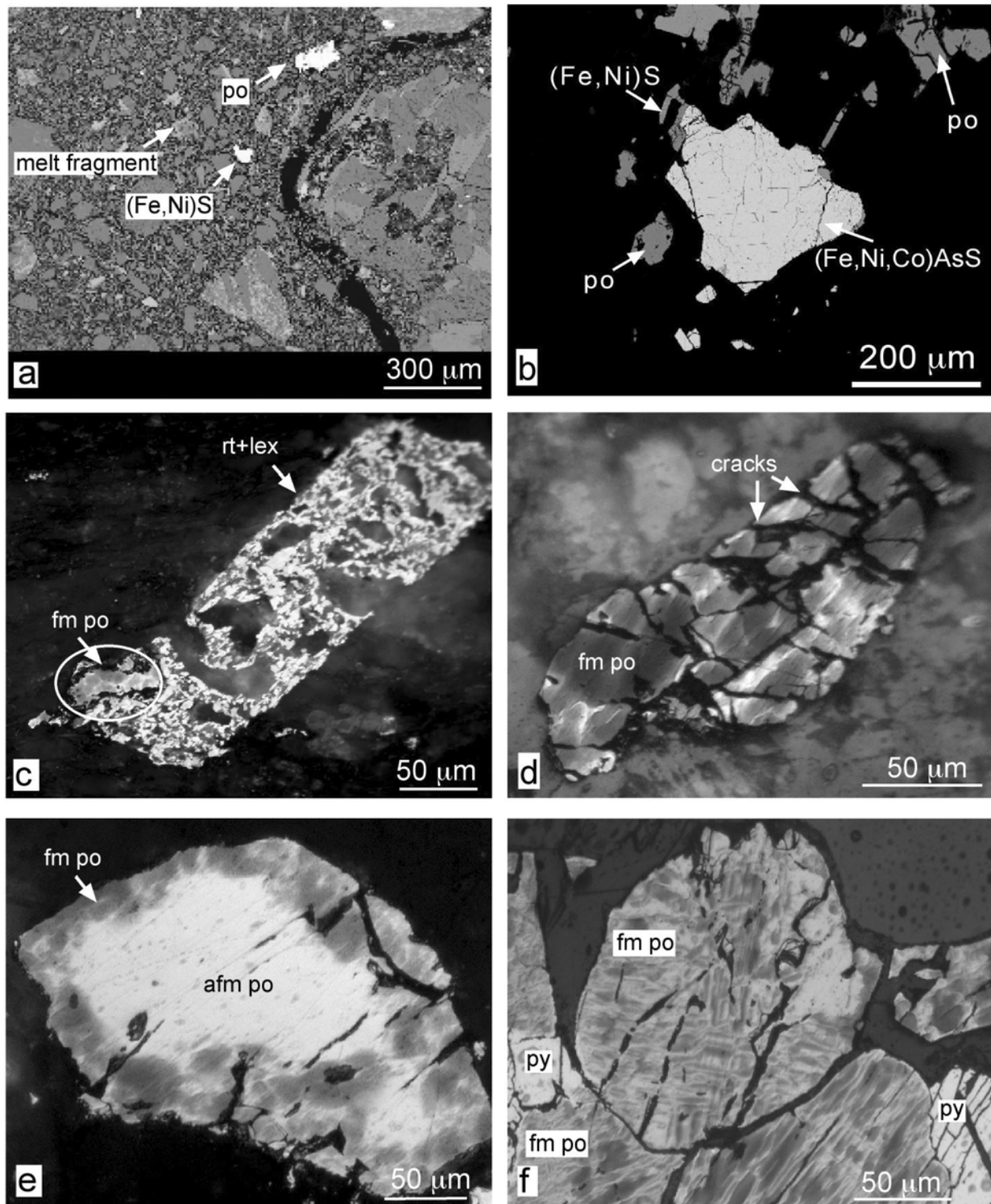
Fig. 1. Photomicrographs with pyrrhotite from different depth and lithology of the LB-07A drill core. a) A BSE image shows the varying size of angular fragments consisting of rock clasts, melt shreds, and mineral grains in a polymict lithic breccia at 354.20 m (po = pyrrhotite). b) A BSE image of pyrrhotite grains associated with millerite [(Fe,Ni)S] and sulfoarsenide [(Fe,Ni,Co)AsS] in a sulfide lens within a greenschist-clast at 376.0 m (polymict breccia unit). c) Ferrimagnetic pyrrhotite (fm po) next to rutile and leucoxene (bright gray) as alteration products of ilmenite in a clast from the suevite at 389.73 m. d) Fractured ferrimagnetic pyrrhotite in a clast from the suevite at 408.49 m. e) Ferrimagnetic pyrrhotite as rim around antiferromagnetic type (afm po). Note the abundant cracks in the grain (polymict lithic breccia, 354.20 m). f) Brecciated ferrimagnetic pyrrhotite in a polymict lithic breccia, 356.32 m. (c to f) are coated with a magnetic colloid to distinguish magnetic from non-magnetic phases.
